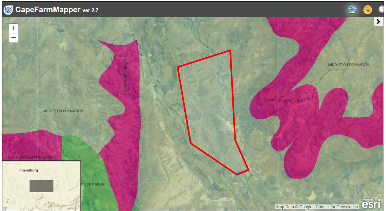
Figure 5-4: Geological formations present on the study site
