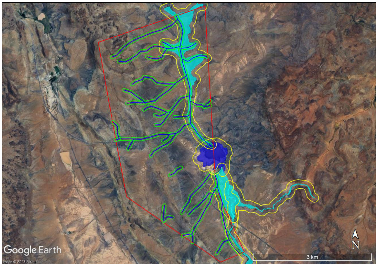
Figure 5-11: Proposed buffers and no-go areas within the Klipkraal WEF phase 4 (yellow lines are 100m and green lines are 40m)
