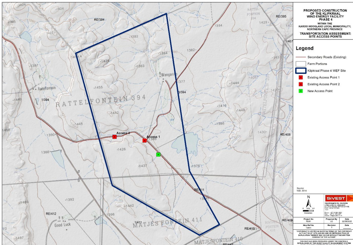
Figure 8.1 Klipkraal WEF 4 - Internal Layouts, also showing site access point
