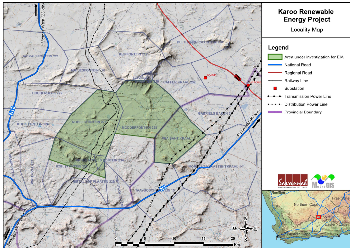
Figure 1-1: Locality map indicating locations of the proposed Karoo Renewable Energy Facility
