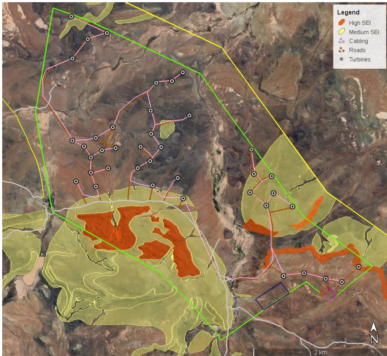
Figure 6. SEI for the Karoo Dwarf Tortoise within the Klipkraal 2 WEF Site.
