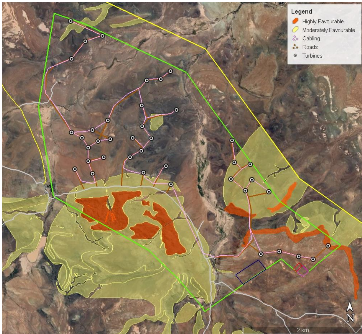
Figure 5. Map of areas considered to represent potentially suitable Karoo Dwarf Tortoise habitat within the Klipkraal 2 WEF site based on ground-truthed mapping from satellite imagery.
