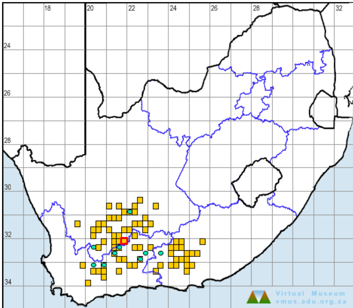
Figure 2. Historical and recent distribution records for the Karoo Dwarf Tortoise according to the Virtual Museum records. The approximate location of the Klipkraal 2 WEF Site is indicated in red.
