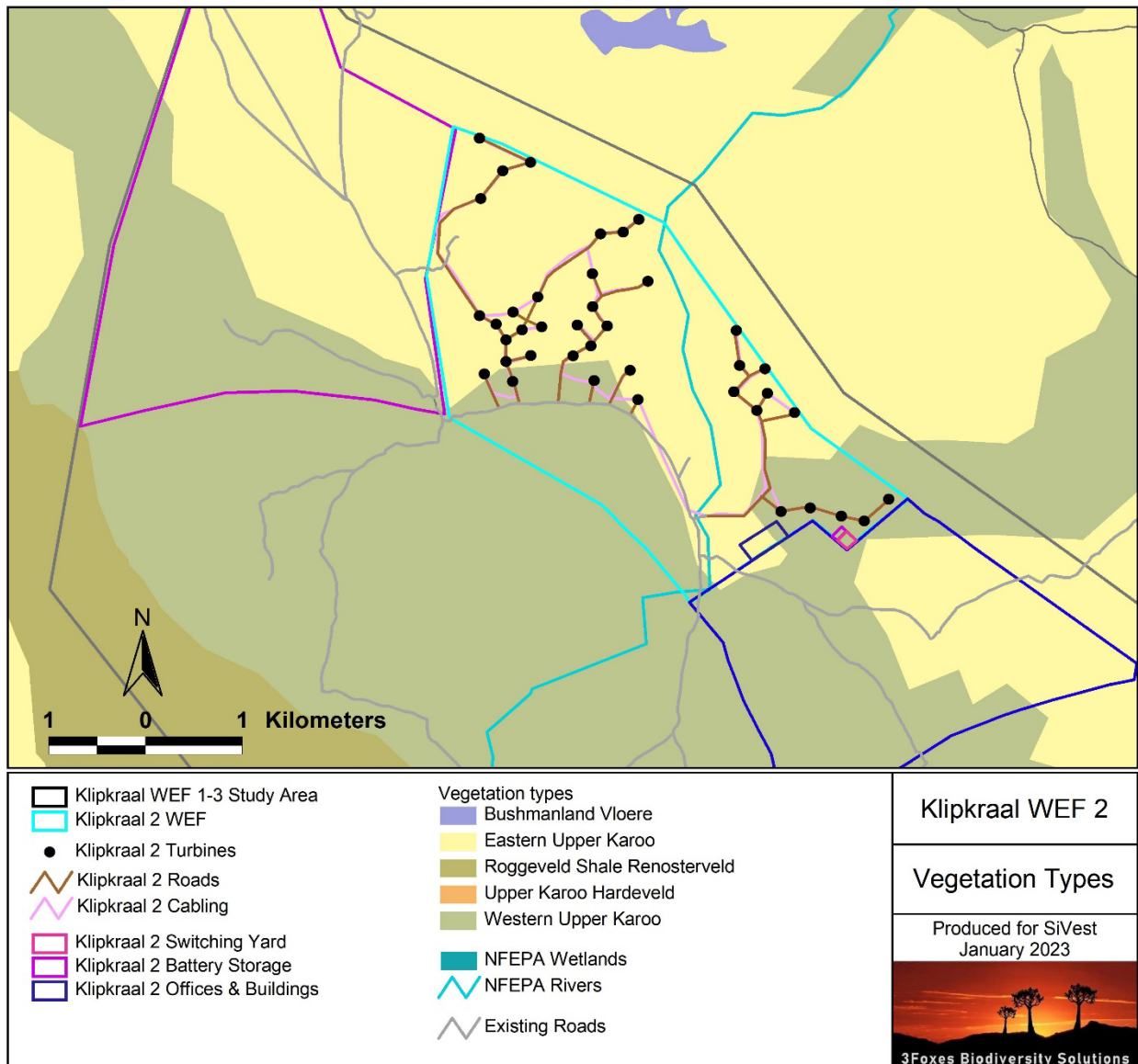
Figure 2. Vegetation map of the Klipkraal 2 WEF project area, showing that the Klipkraal 2 site falls within the Eastern Upper Karoo and Western Upper Karoo vegetation types.
