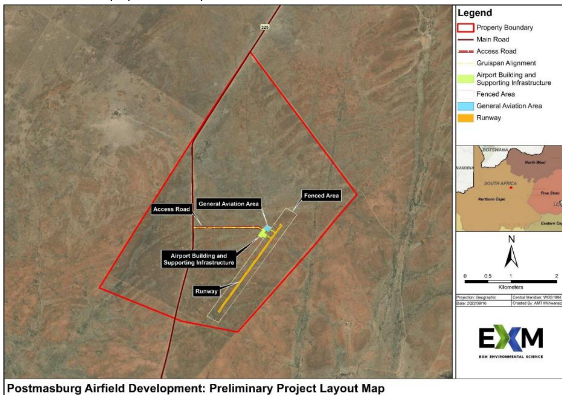
Figure 1b: Preliminary project lay-out plan (APelser).
