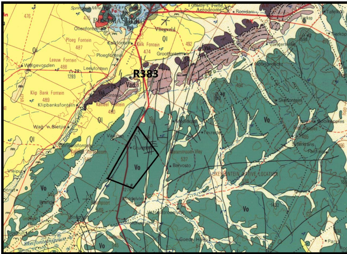
Figure: Regional geology of the development.
