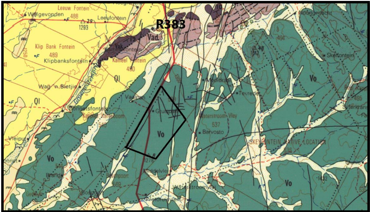
Figure 3: Geology of the area (Moen 1977b) (1h).
