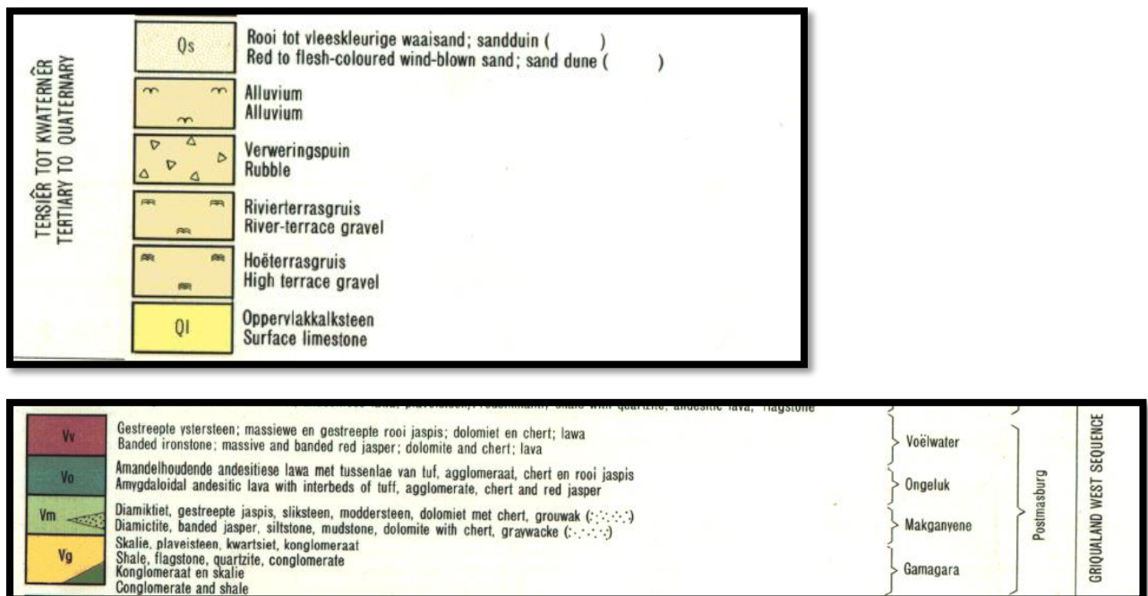
Figure 4: Lithology (Moen 1977b).
