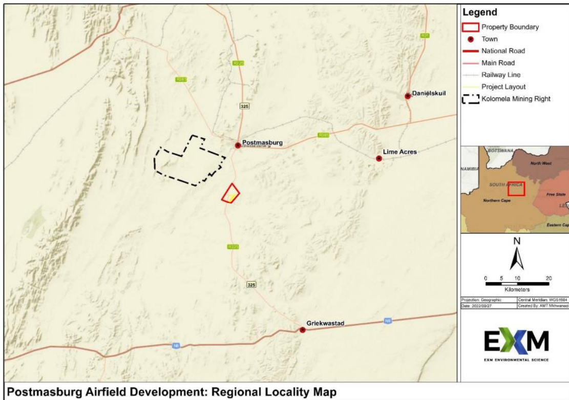
Figure 1a: Regional map showing locality (APelser).
