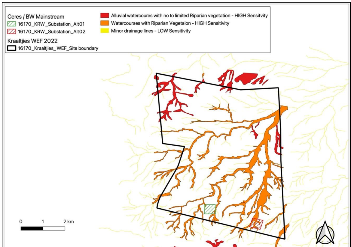
Figure 11: Delineated aquatic zones and respective sensitivities
