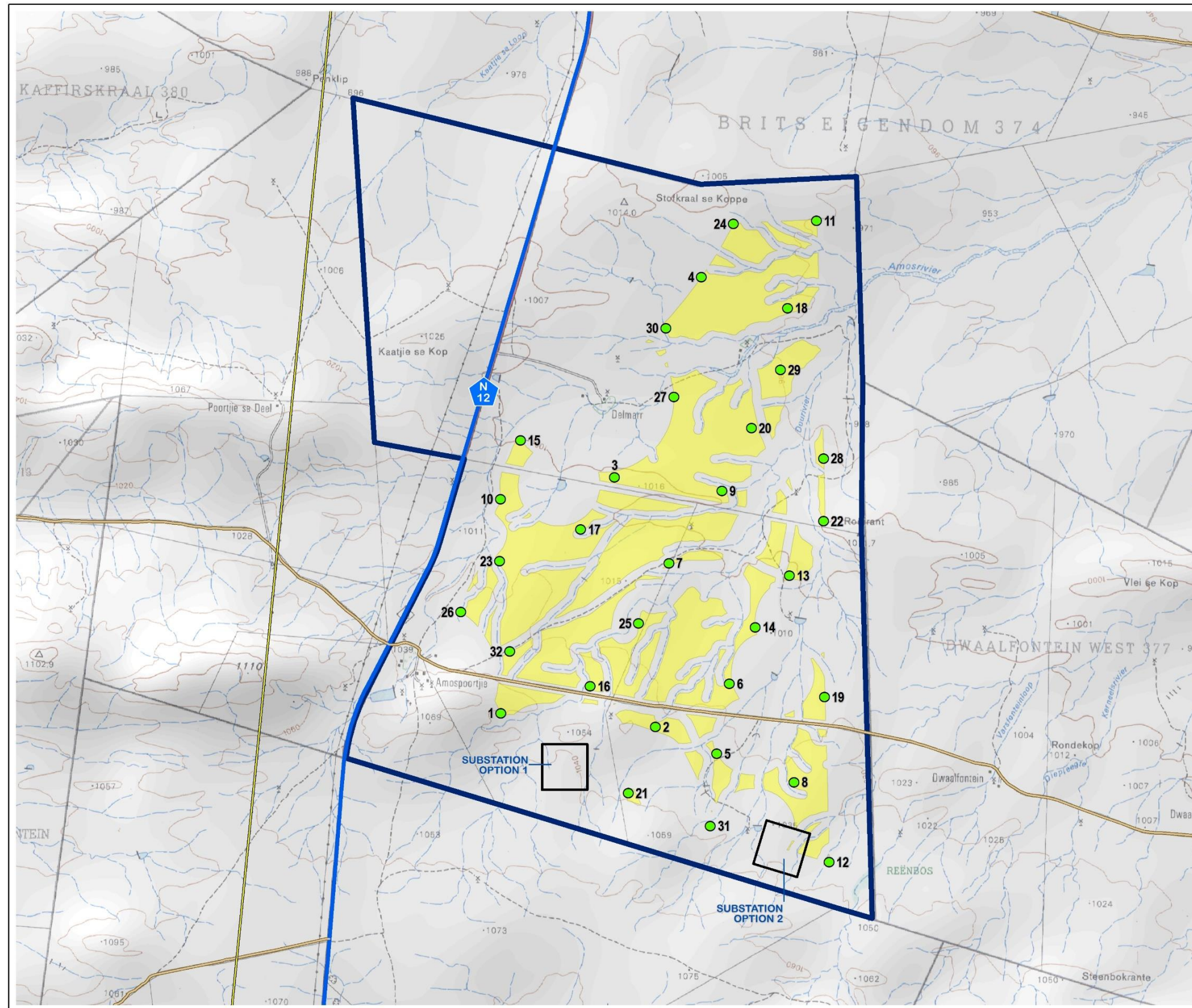
MAP 3: Preliminary WEF Layout
