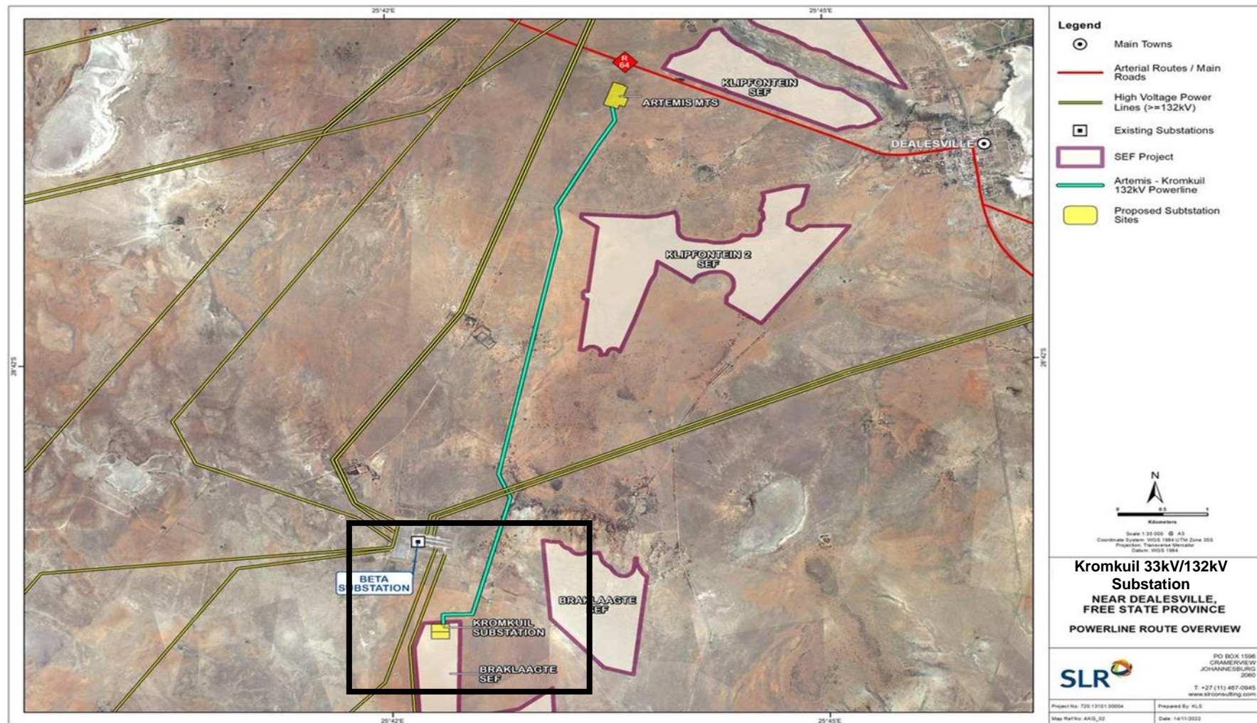
Figure 3: Layout map for the proposed Kromkuil onsite substation in relation to the authorised Artemis MTS
