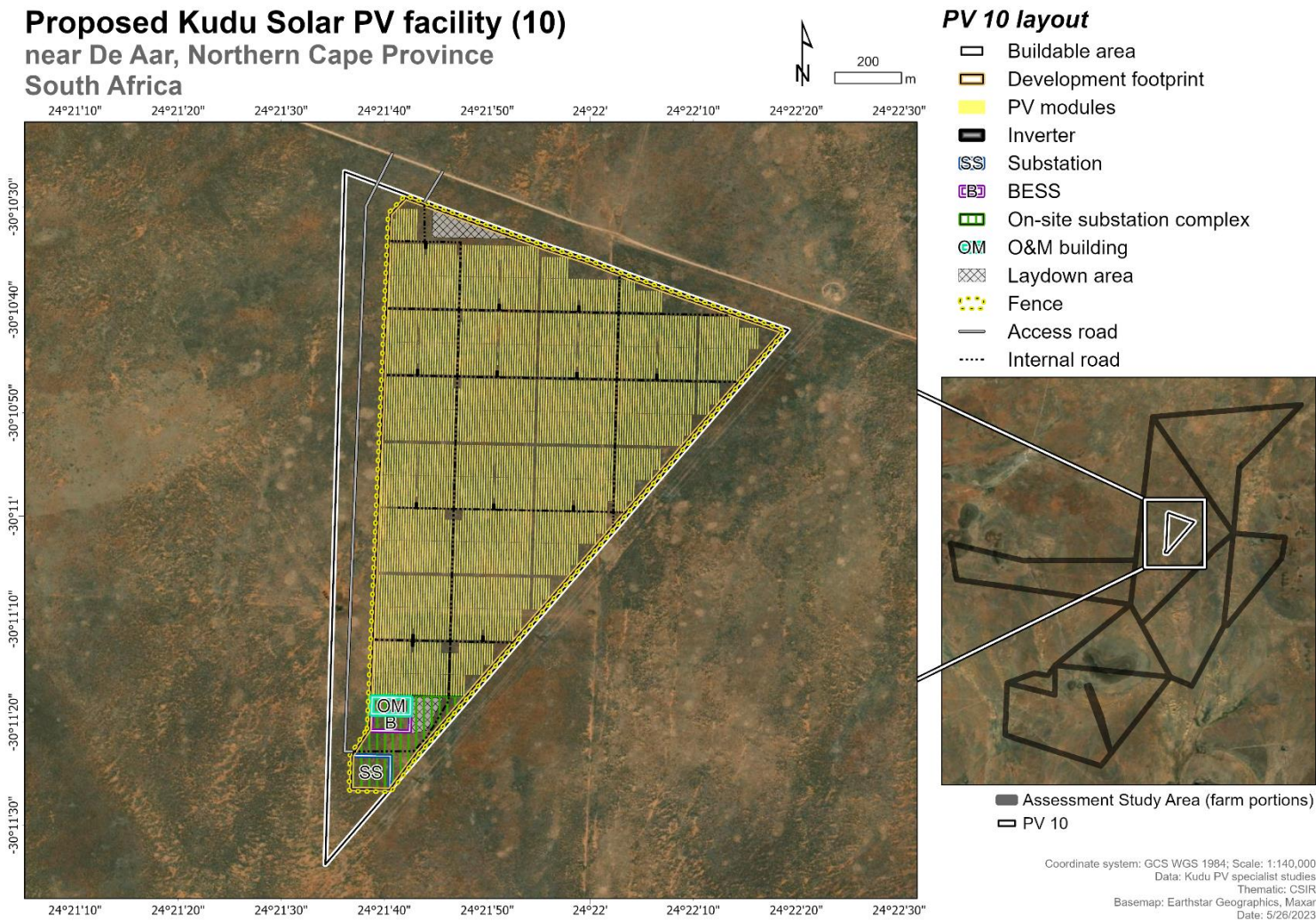
Map 17-6: Detailed layout of Kudu Solar Facility 10.
