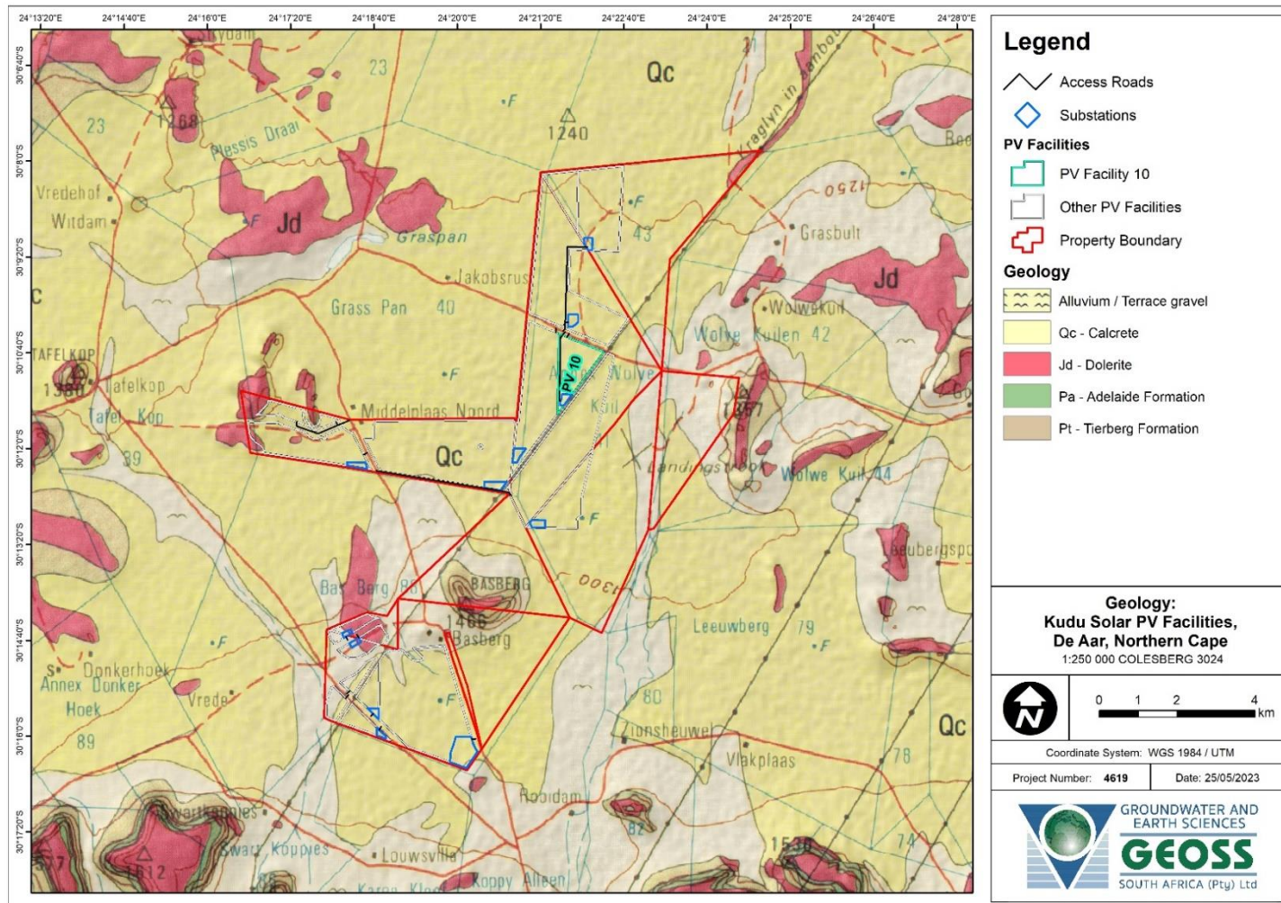
Map 17-3: Geological setting of the study area for the 12 Kudu Solar Facilities. Note that this report is focused on Kudu Solar Facility 10.
