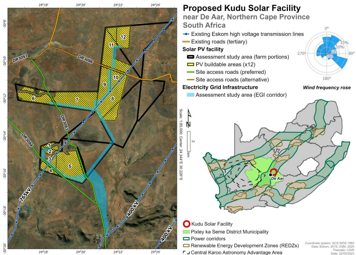
Figure 1.1: Location of the Kudu PV4 SEF within the SEF cluster
