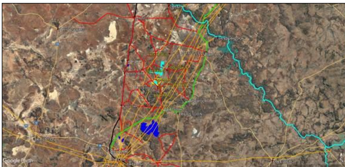
Figure 3.4: Kudu 4 PV site property (yellow outline) in relation to other proposed Kudu 1-12 PV sites (light blue fill), settlements, provincial boundaries (light blue lines), existing transmission lines (orange), the R48 (green) and study area gravel road network (red), railway line (black) and operational REFs (dark blue fill).
