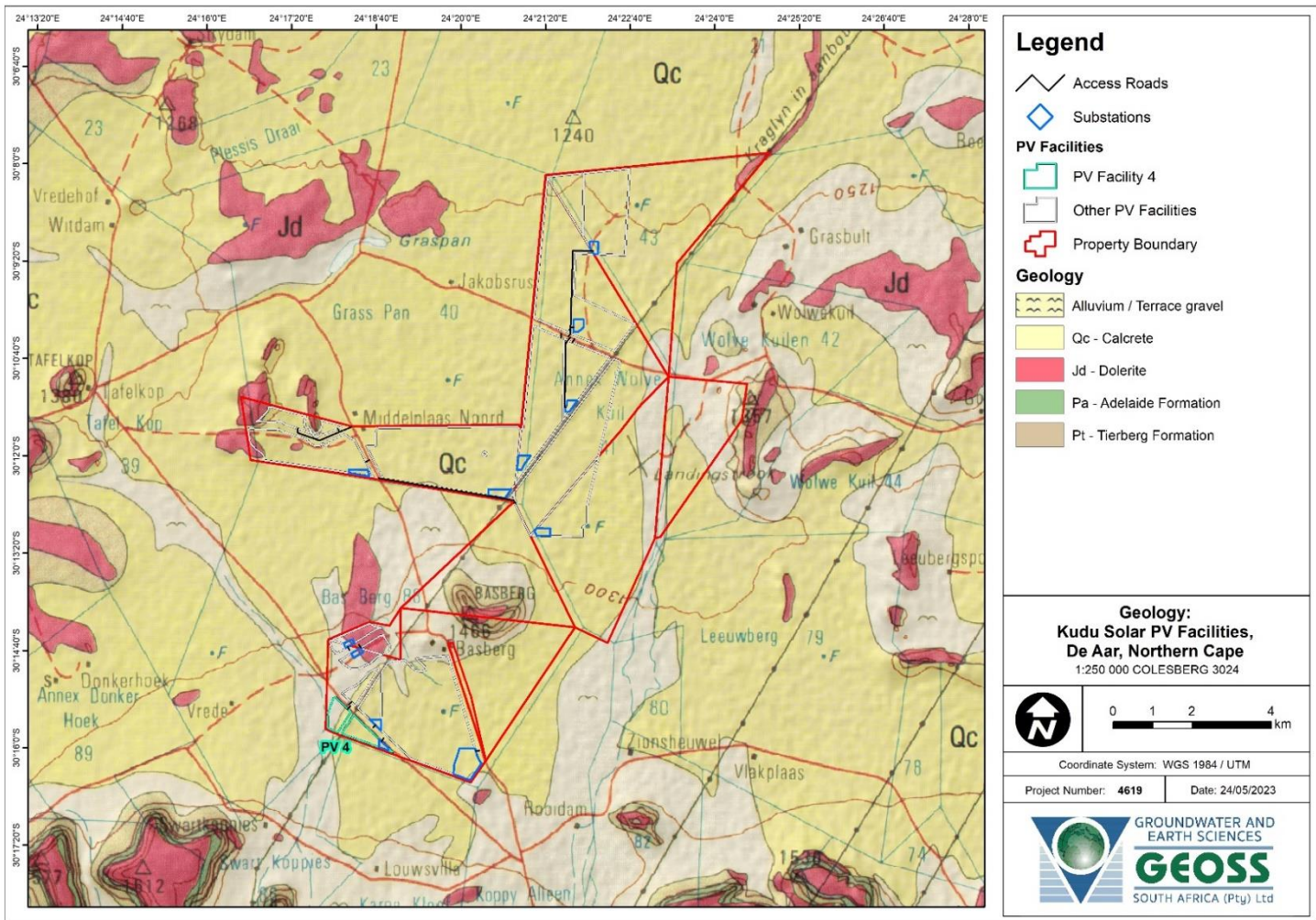
Map 17-3: Geological setting of the study area for the 12 Kudu Solar Facilities. Note that this report is focused on Kudu Solar Facility 4.
