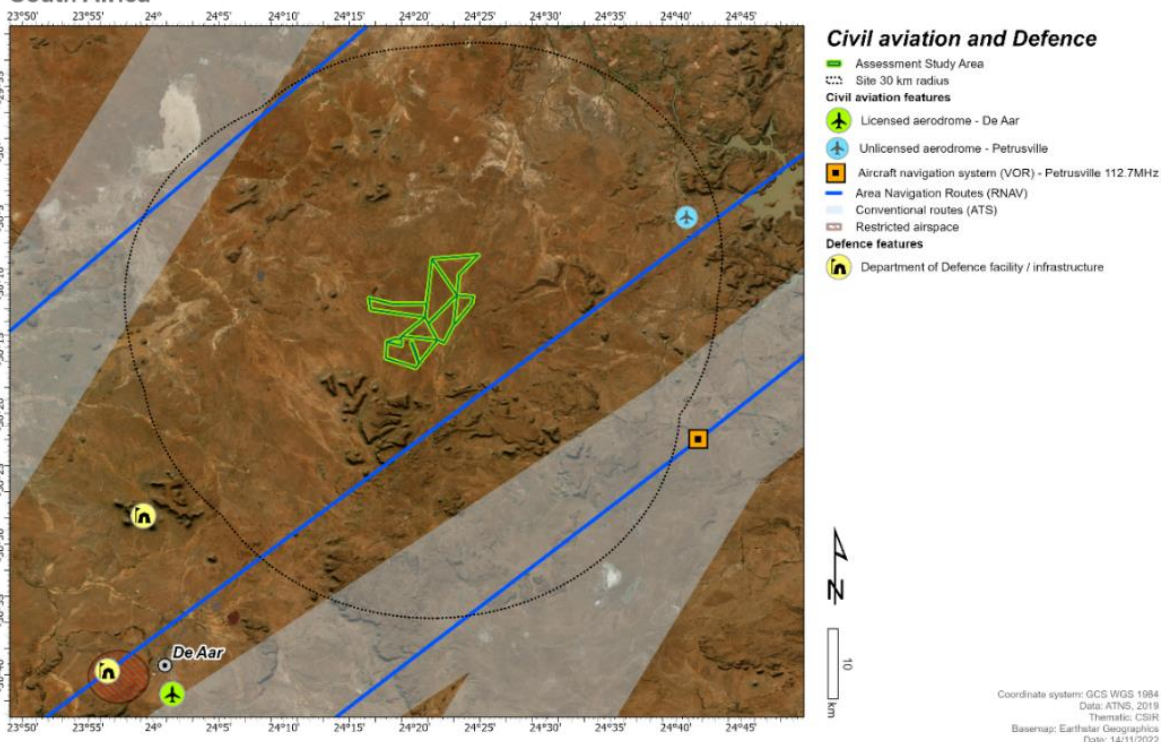
Figure 18-7: Civil Aviation features relative to the proposed project study area based on the site visit and existing databases.
