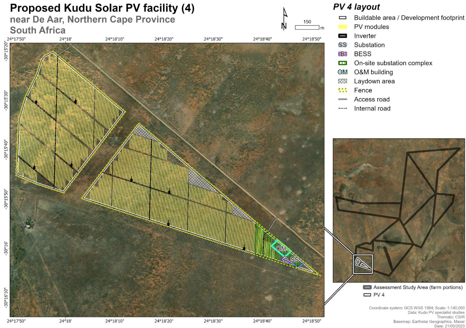
Map 17-6: Detailed layout of Kudu Solar Facility 4.
