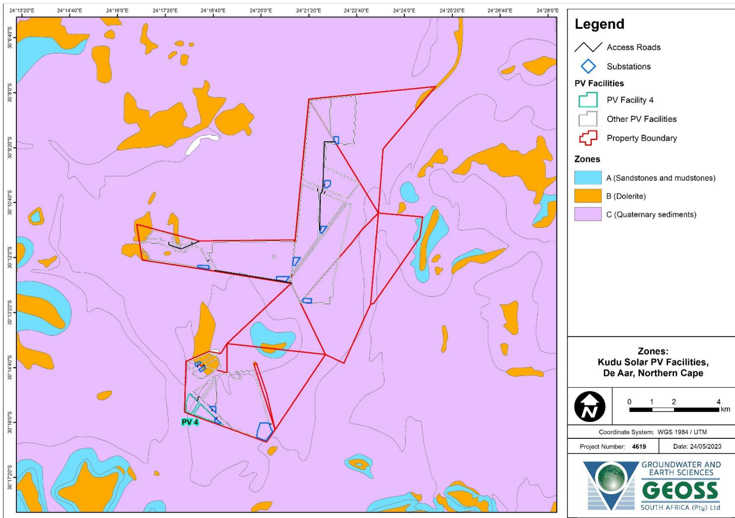
Map 17-4: Broad geotechnical zones across the study area. Note that this report is focused on Kudu Solar Facility 4.
