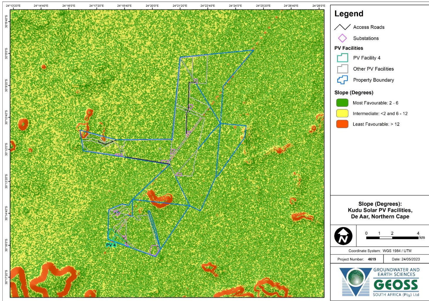
Map 17-5: Regional slope classification based on Stiff et al. (1996). Note that this report is focused on Kudu Solar Facility 4.
