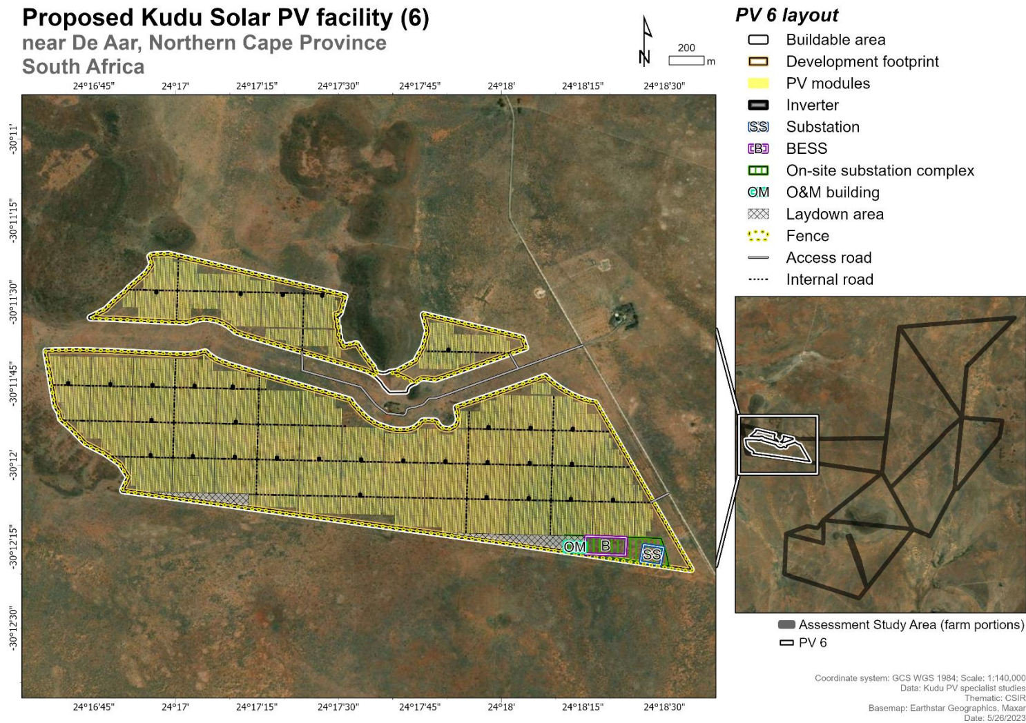
Map 17-6: Detailed layout of Kudu Solar Facility 6.
