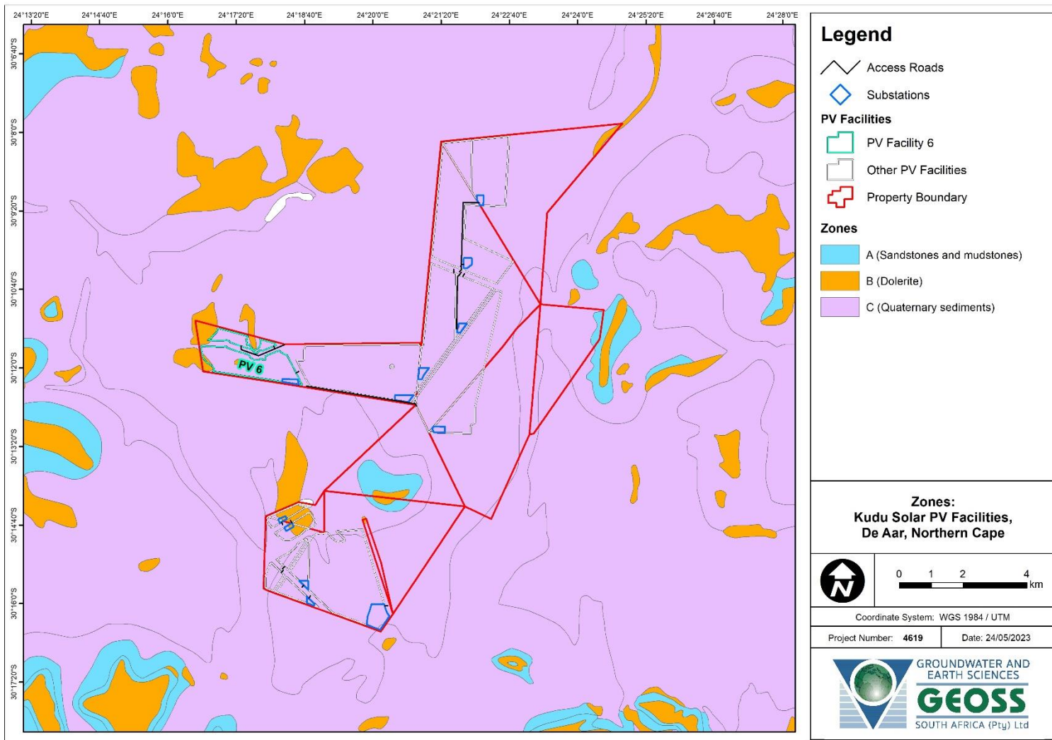
Map 17-4: Broad geotechnical zones across the study area. Note that this report is focused on Kudu Solar Facility 6.
