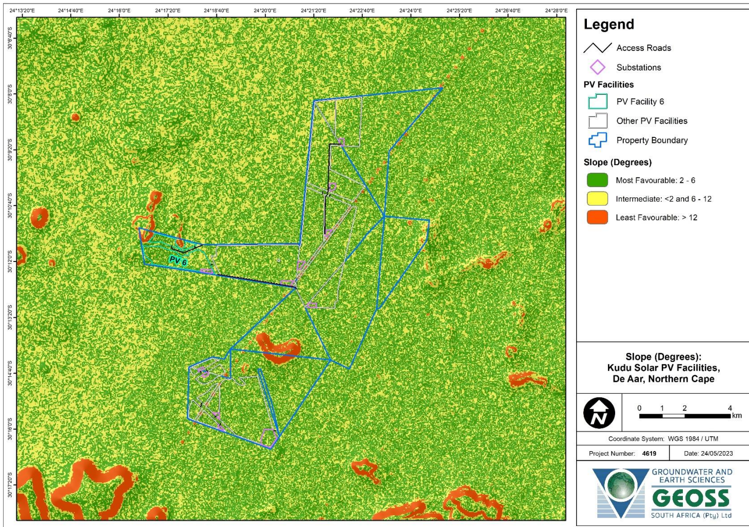
Map 17-5: Regional slope classification based on Stiff et al. (1996). Note that this report is focused on Kudu Solar Facility 6.
