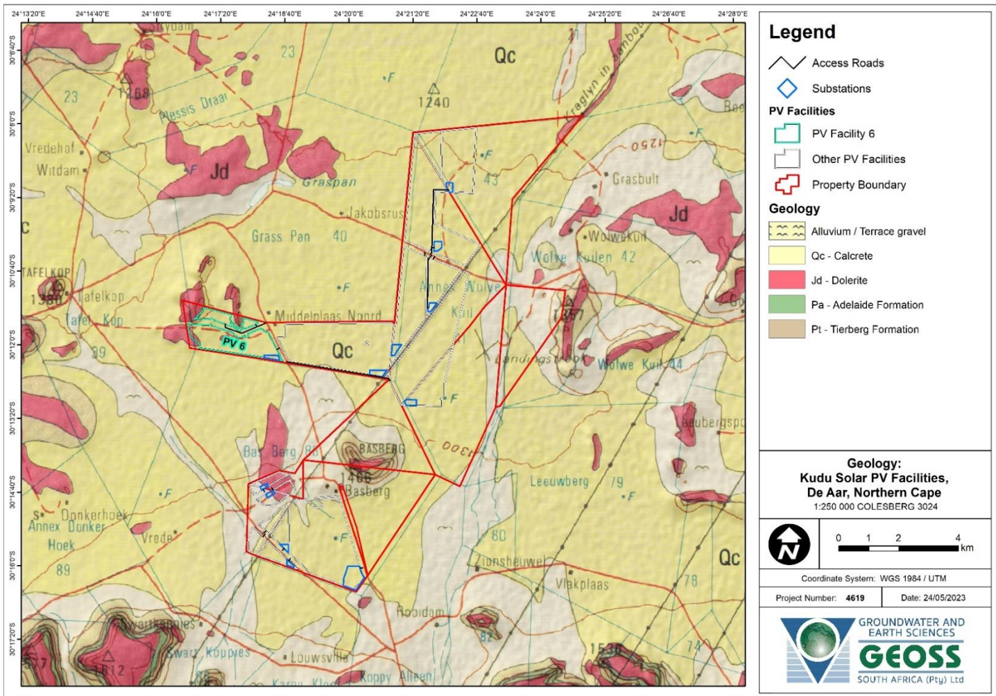
Map 17-3: Geological setting of the study area for the 12 Kudu Solar Facilities. Note that this report is focused on Kudu Solar Facility 6.
