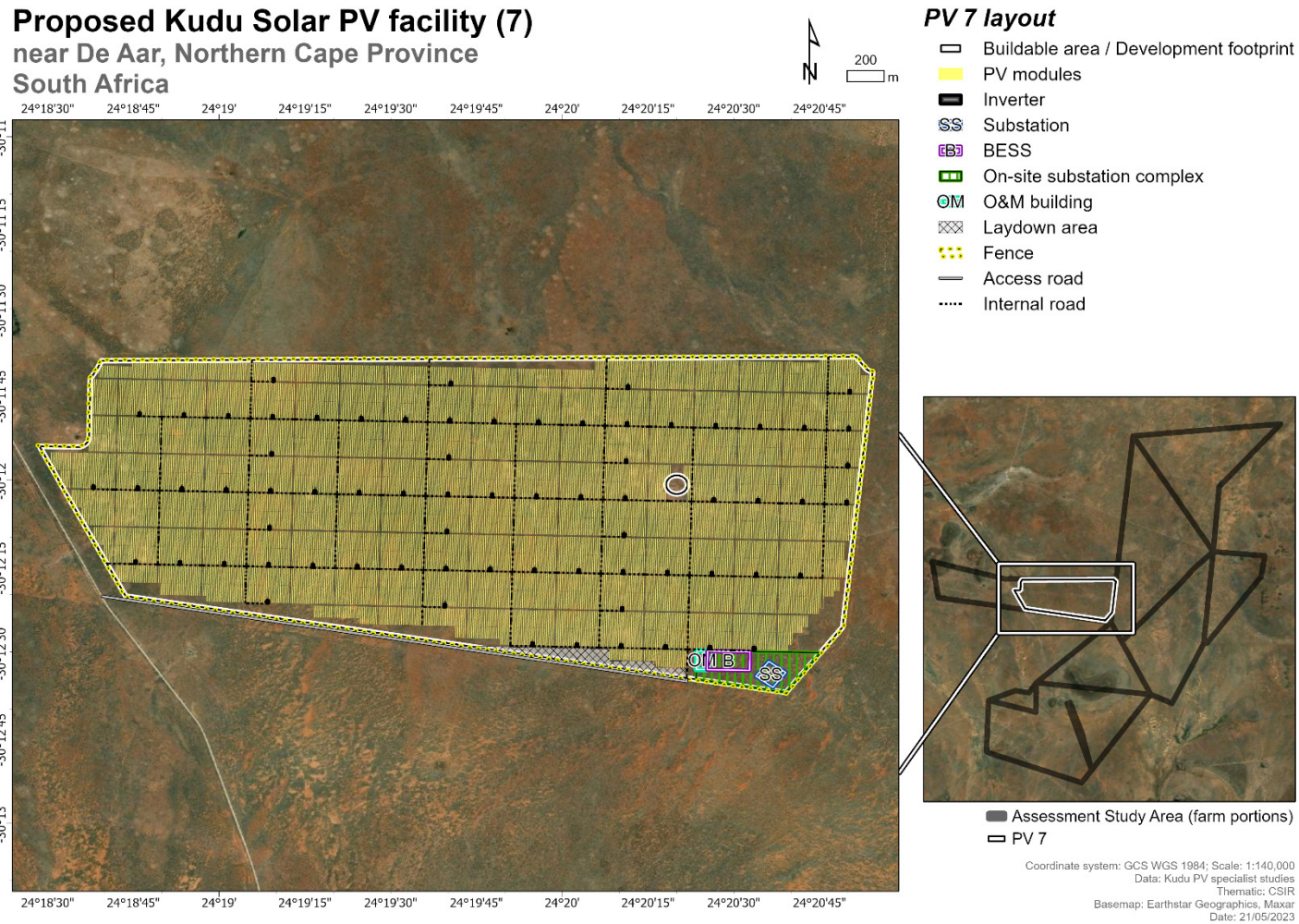
Map 16-9: Detailed Layout of Kudu Solar Facility 7.
