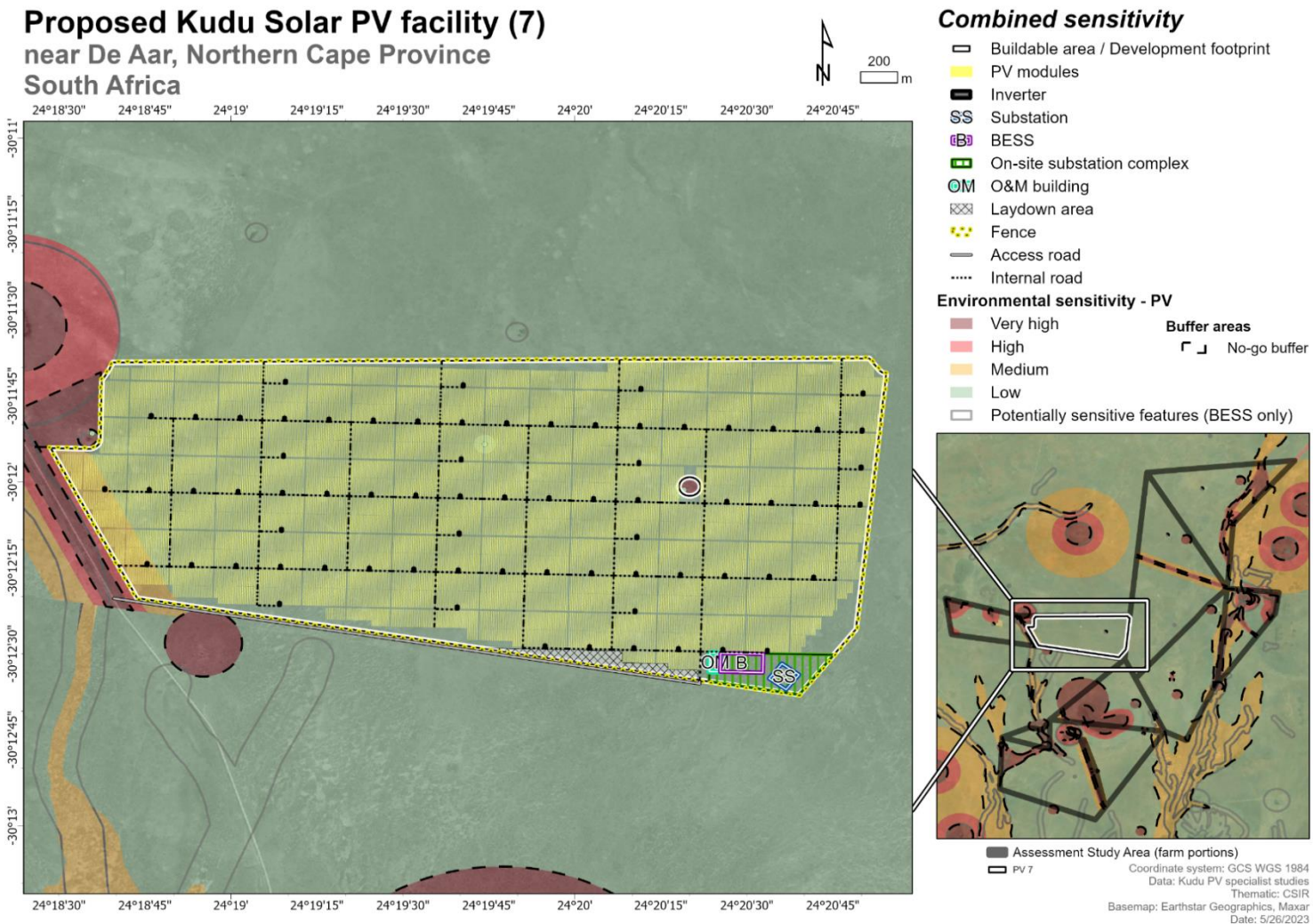
Figure 20-4: Combined Project Layout and Sensitivity Map.
