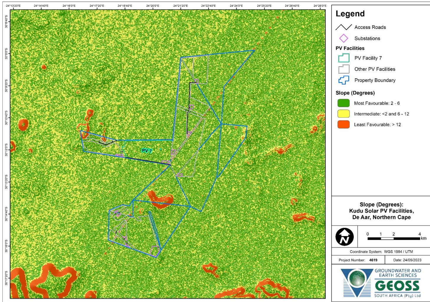
Map 17-5: Regional slope classification based on Stiff et al. (1996). Note that this report is focused on Kudu Solar Facility 7.
