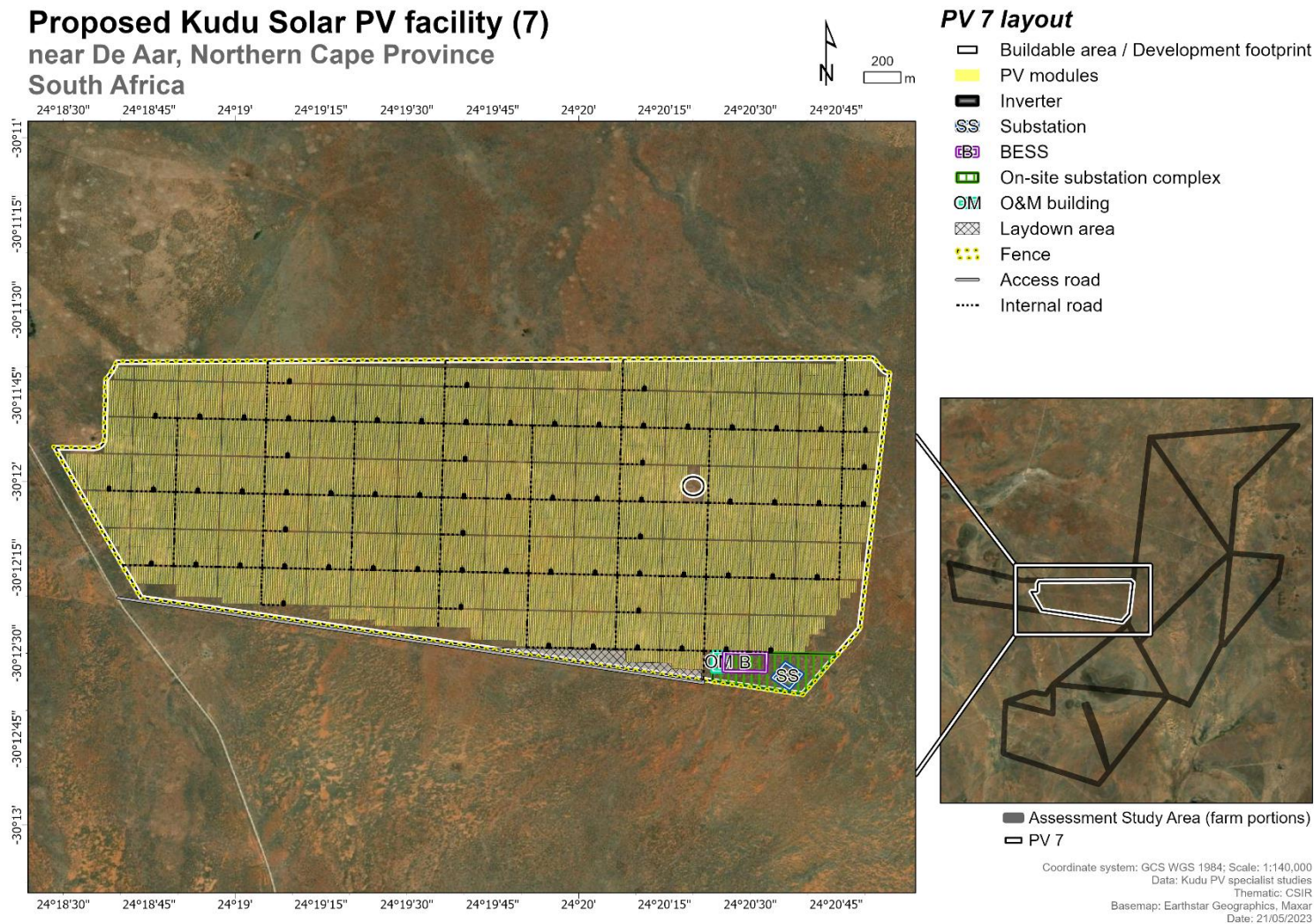
Map 17-6: Detailed layout of Kudu Solar Facility 7.
