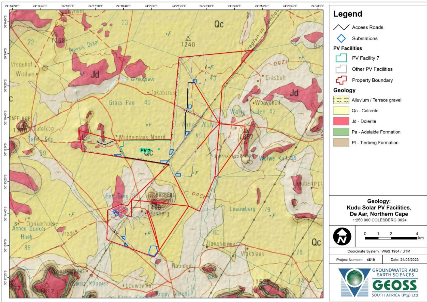
Map 17-3: Geological setting of the study area for the 12 Kudu Solar Facilities. Note that this report is focused on Kudu Solar Facility 7.
