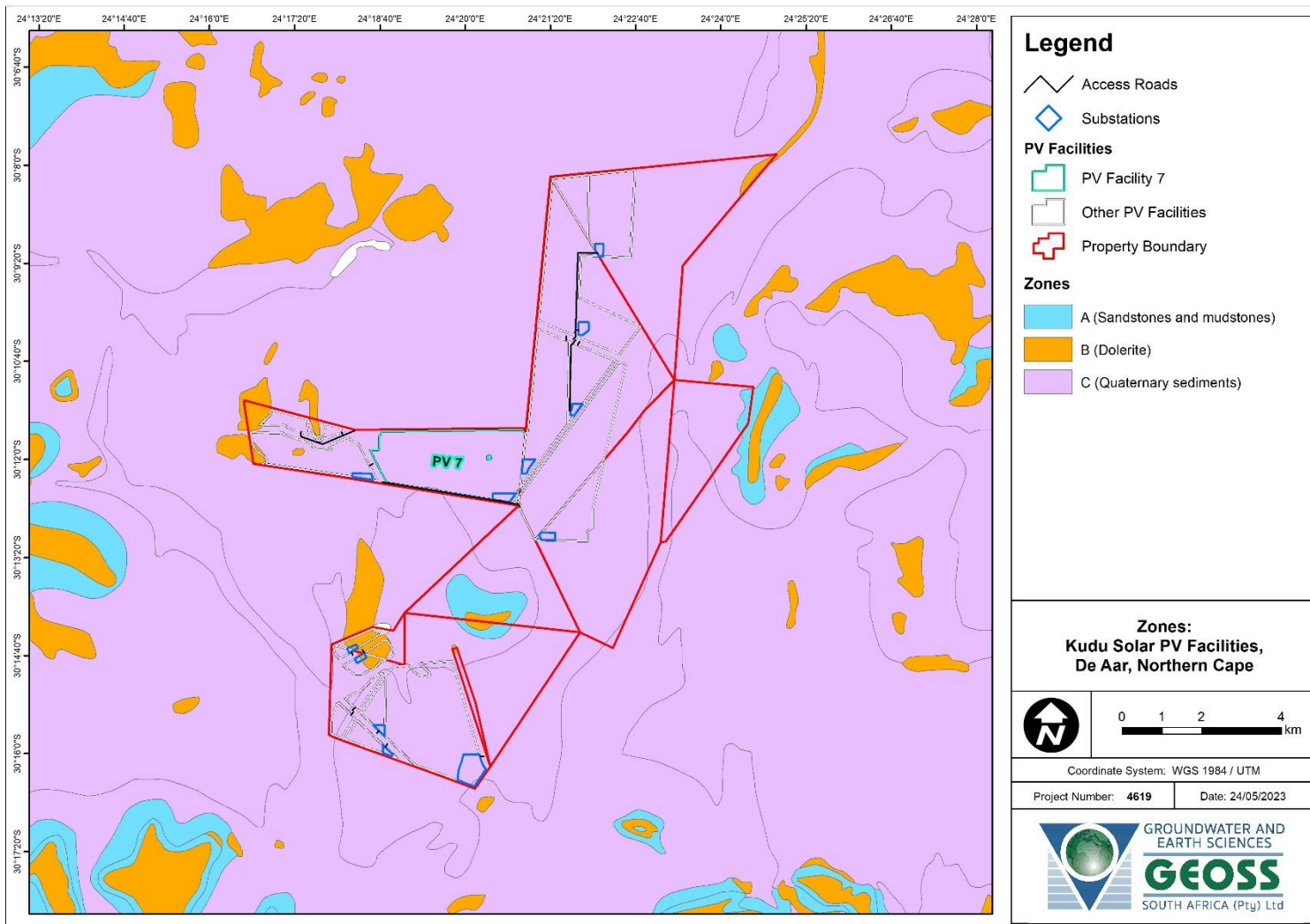
Map 17-4: Broad geotechnical zones across the study area. Note that this report is focused on Kudu Solar Facility 7.
