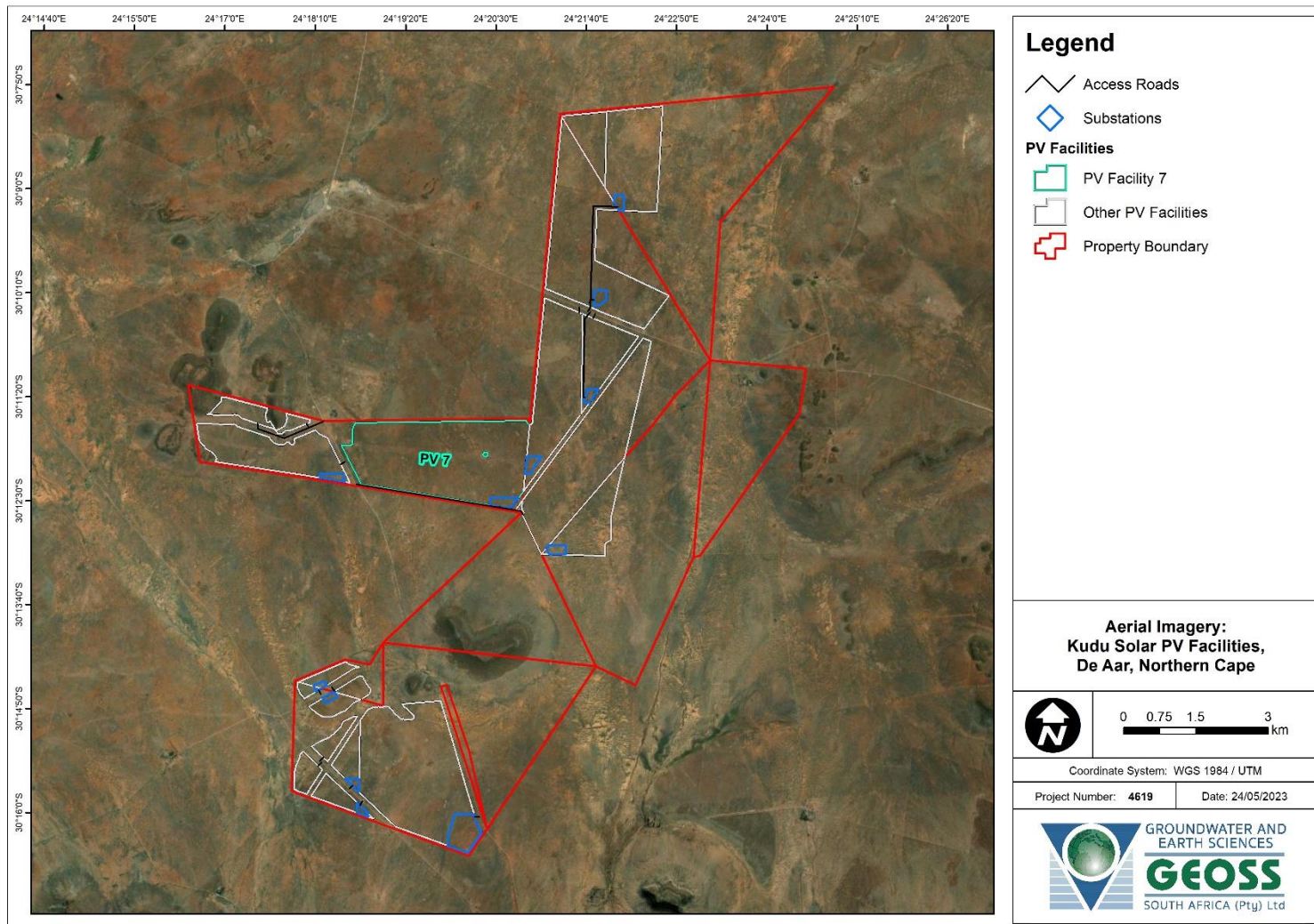
Map 17-2: Aerial view delineating the study area of the 12 Kudu Solar Facilities (Google, 2022). Note that this report is focused on Kudu Solar Facility 7.
