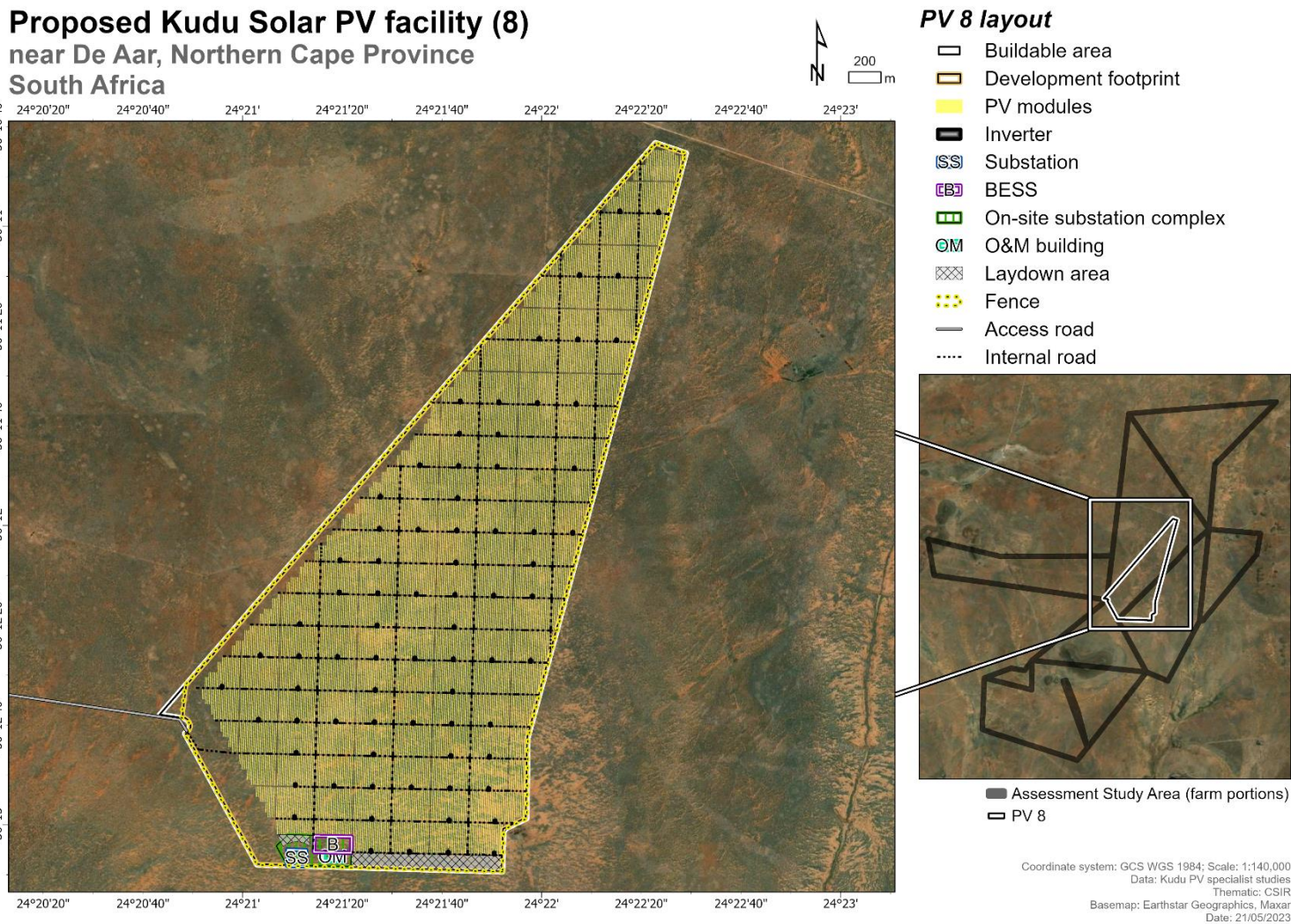
Map 17-6: Detailed layout of Kudu Solar Facility 8.
