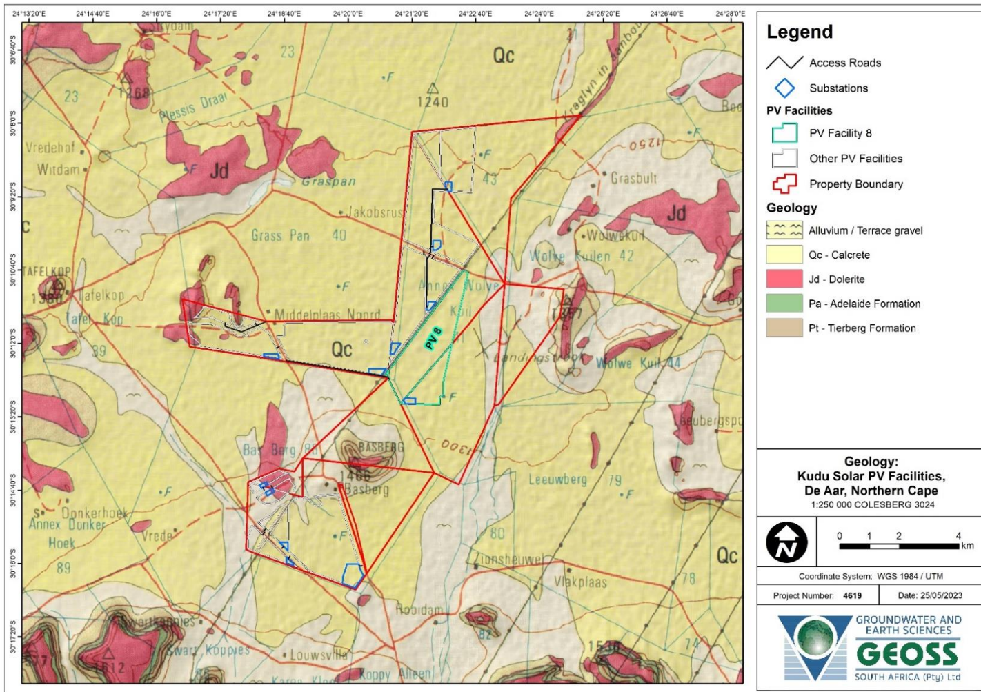
Map 17-3: Geological setting of the study area for the 12 Kudu Solar Facilities. Note that this report is focused on Kudu Solar Facility 8.
