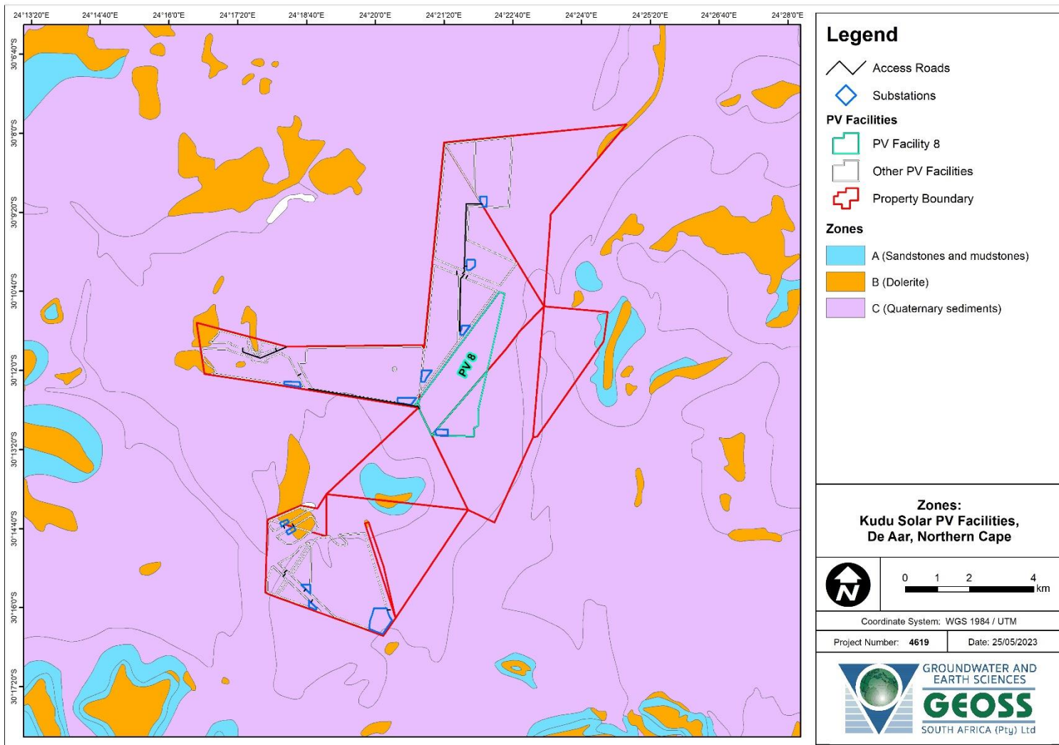
Map 17-4: Broad geotechnical zones across the study area. Note that this report is focused on Kudu Solar Facility 8.
