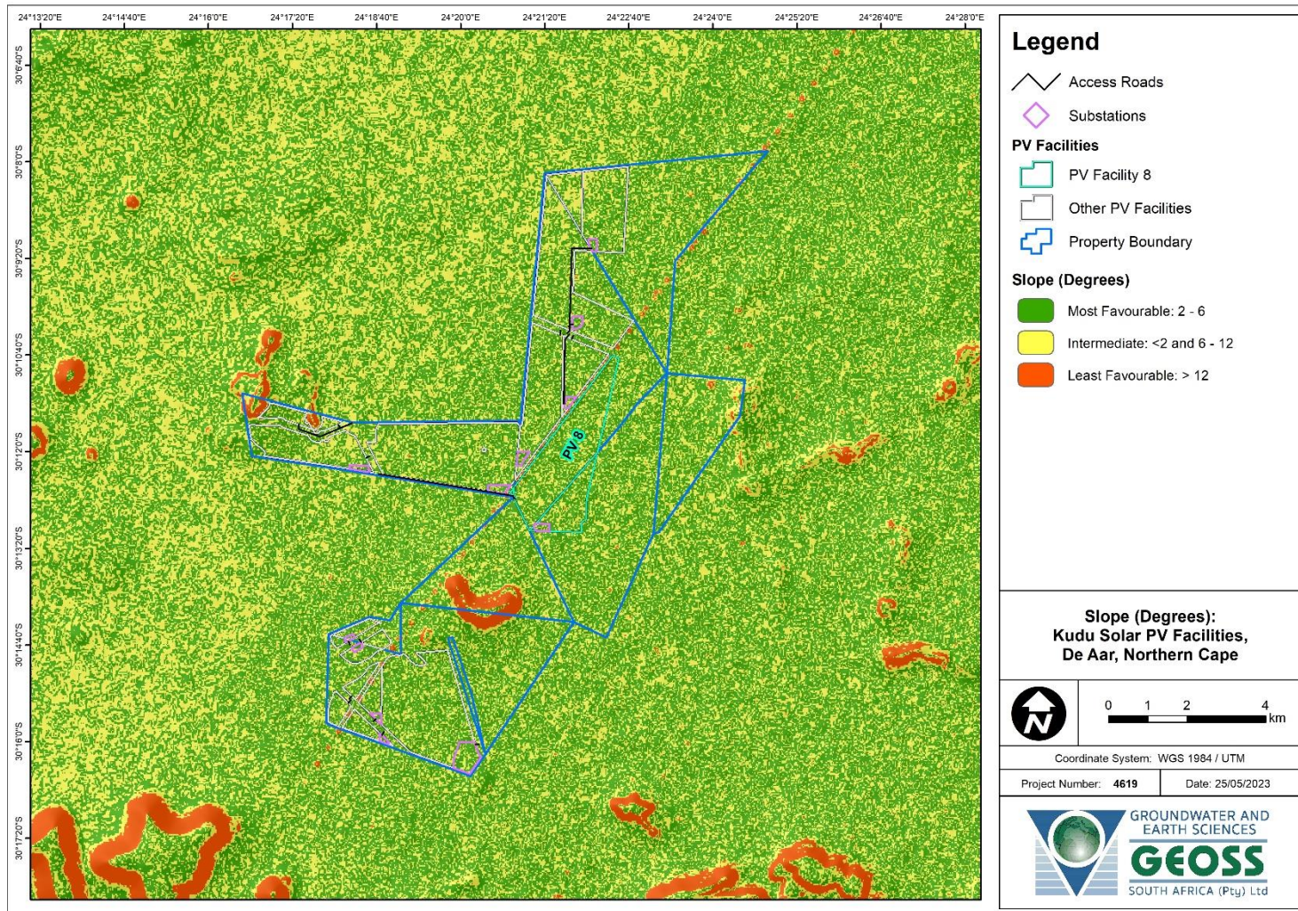
Map 17-5: Regional slope classification based on Stiff et al. (1996). Note that this report is focused on Kudu Solar Facility 8.
