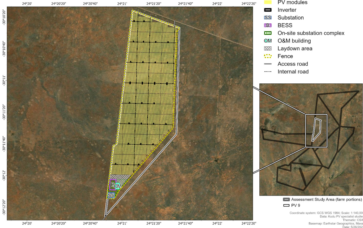
Map 16-9: Detailed Layout of Kudu Solar Facility 9
