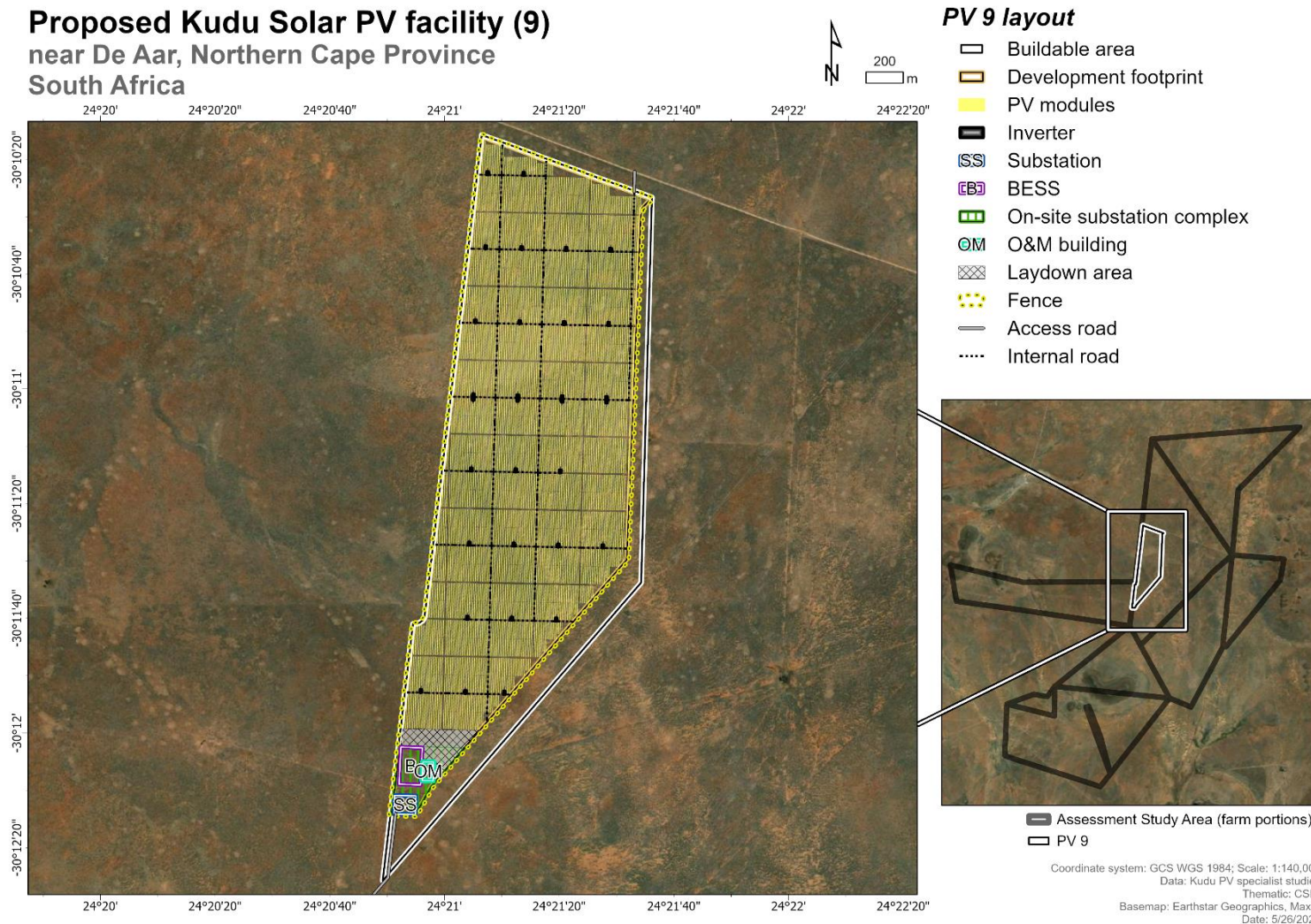
Map 17-6: Detailed layout of Kudu Solar Facility 9.
