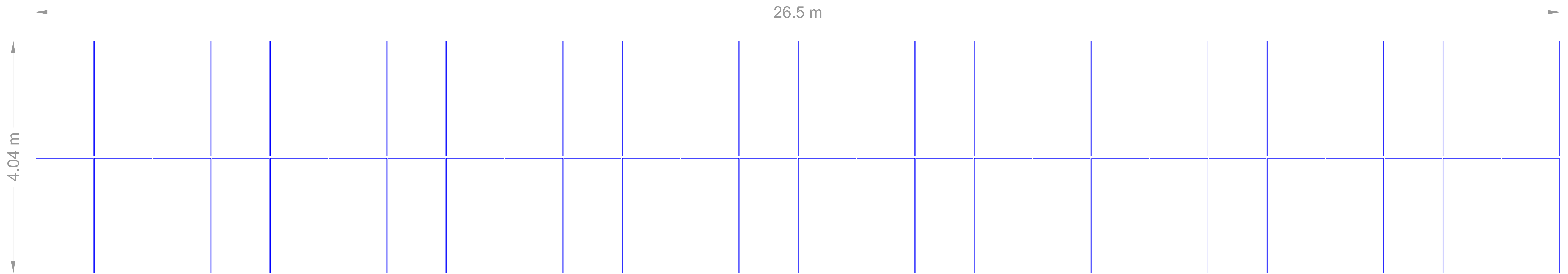
Horizontal projection - scale 1:30 2 x 27 PV modules - portrait orientation 1 PV string = 26 modules in series
