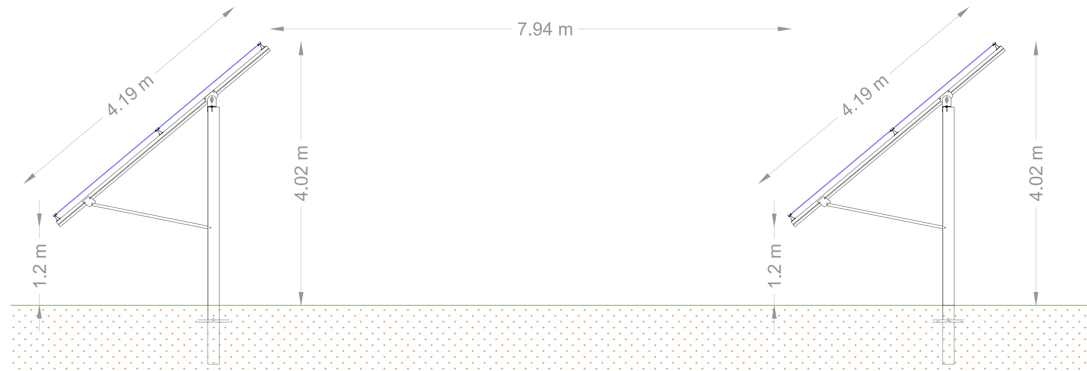
Lateral view - scale 1:30
