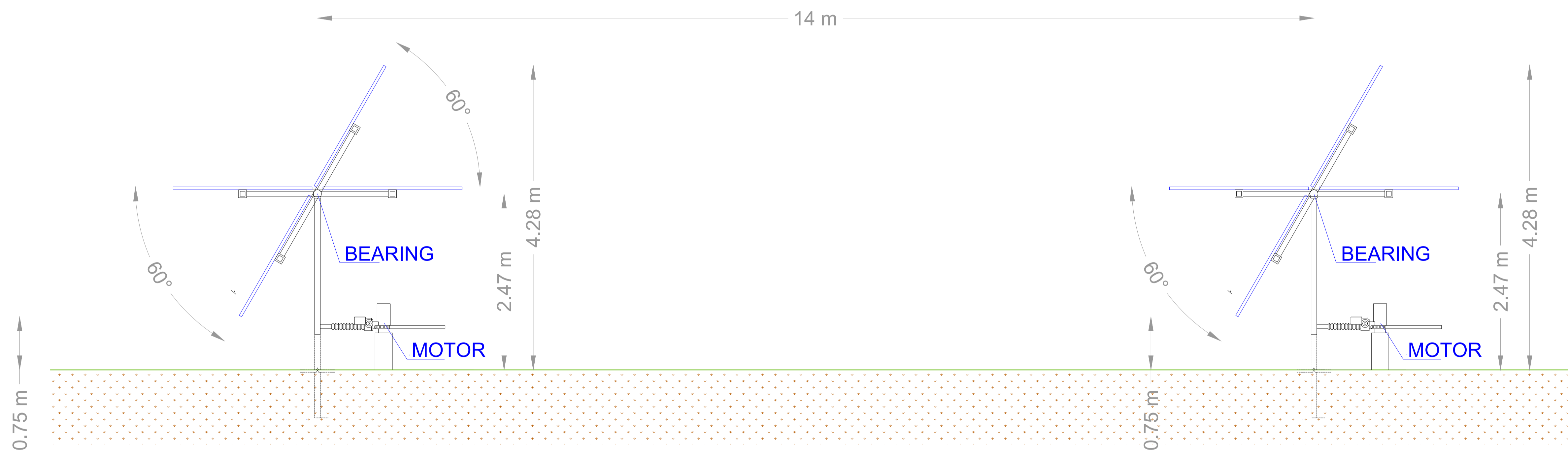
Lateral view - scale 1:30
