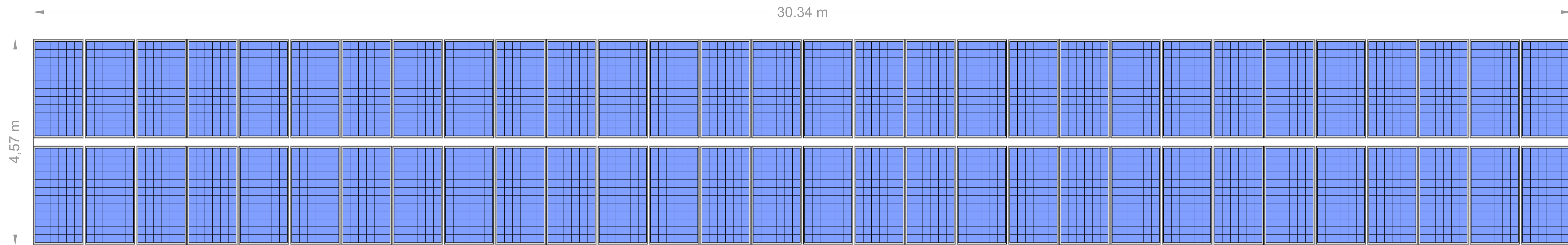
Horizontal projection - scale 1:40 2 x 30 PV modules - portrait orientation 1 PV string = 30 modules in series
