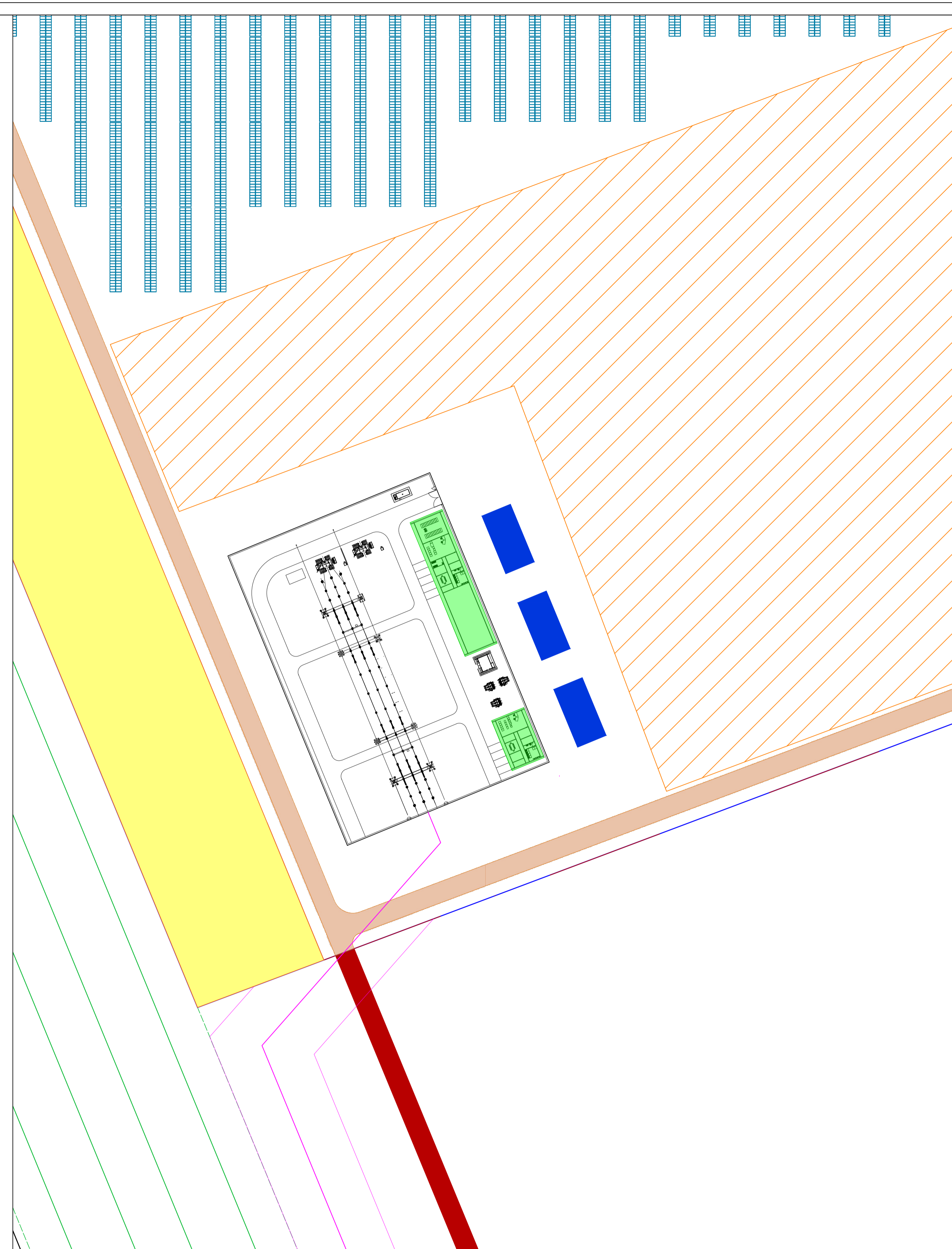
On-site 33kV/132kV substation, switching station and control buildings SCALE 1:1.000
