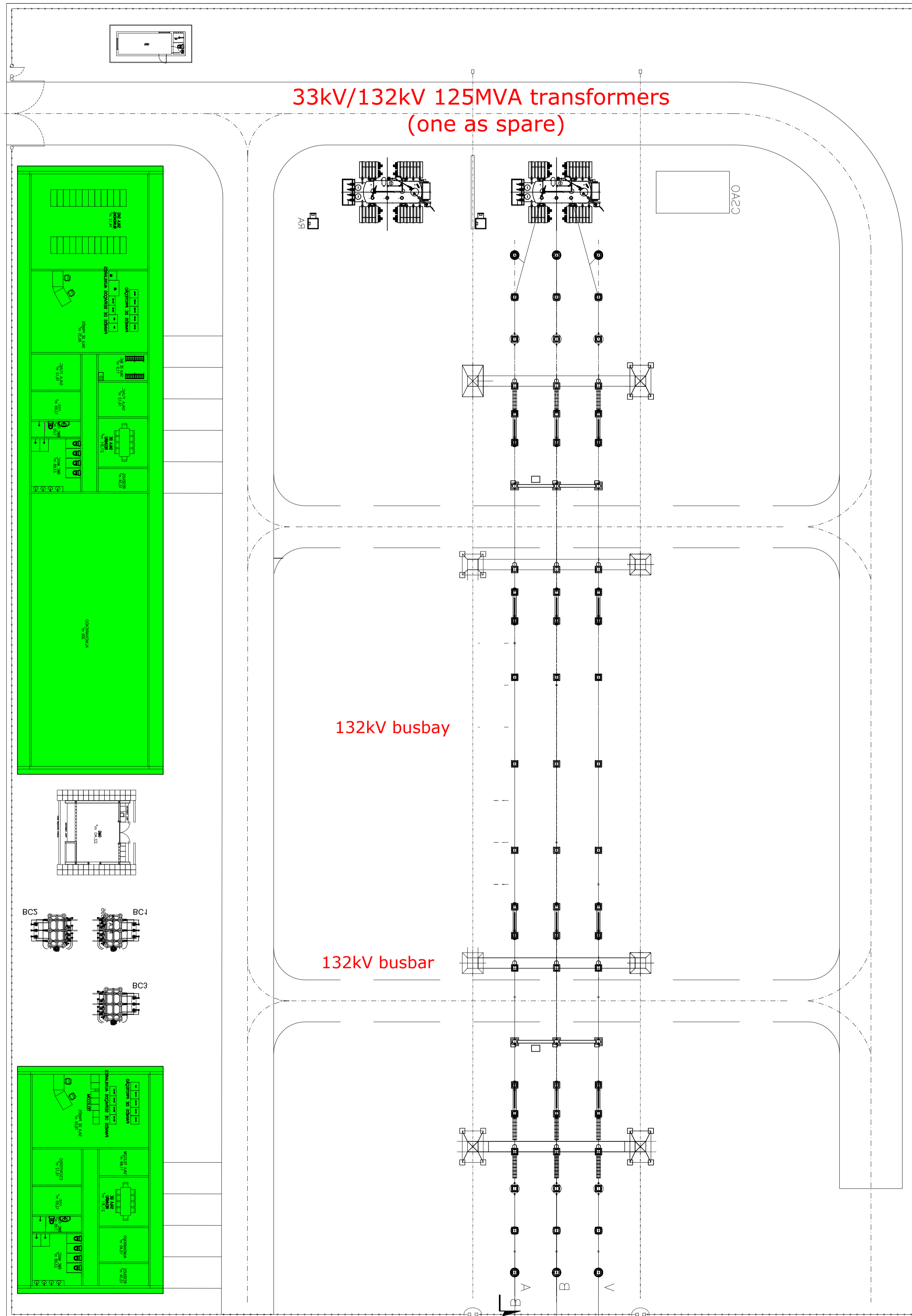
On-site 33kV/132kV step-up substation, switching station and control buildings SCALE 1:250
