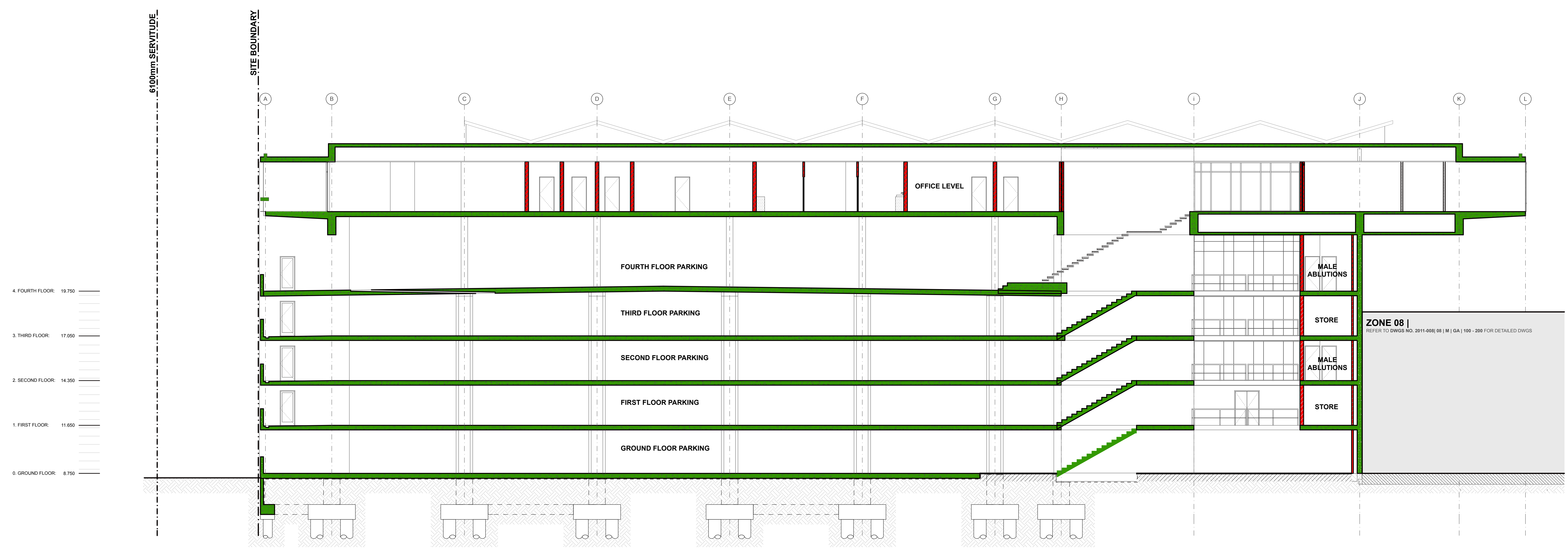
SECTION | A - A SCALE 1:100
