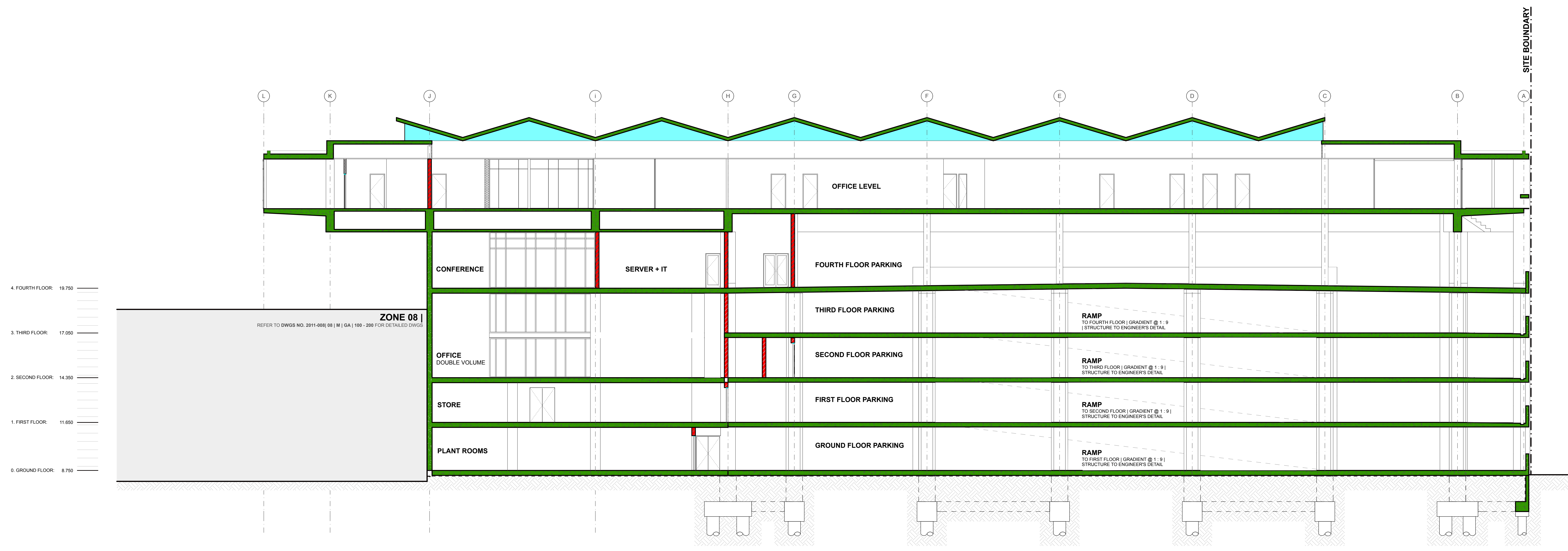
SECTION | B - B SCALE 1:100
