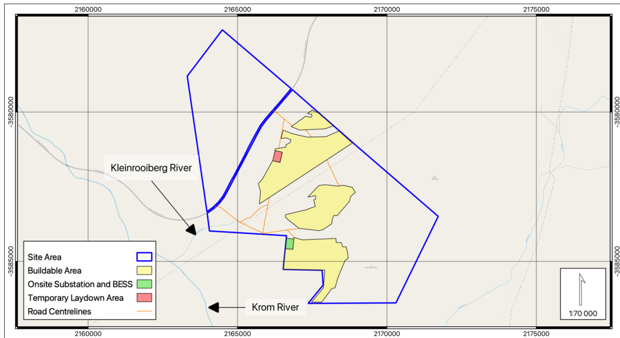
Figure 3-2 Development layout plan of Lesaka SEF 1
