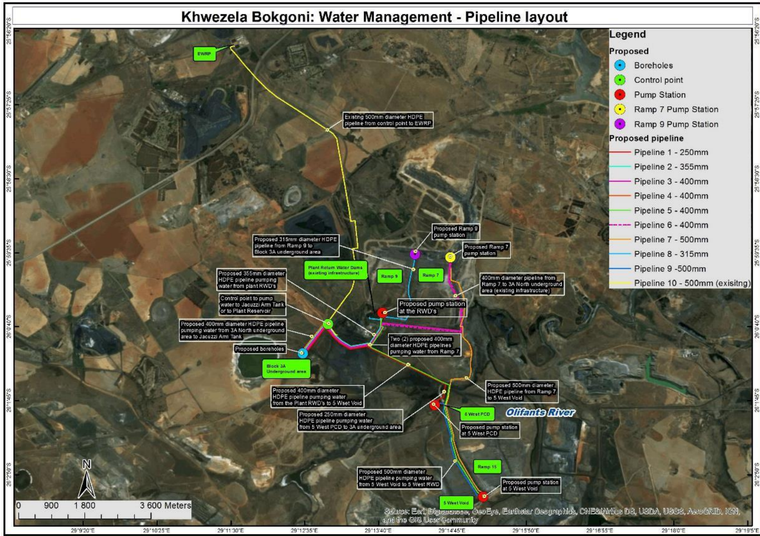
Figure 2: Layout Map of the proposed activities.
