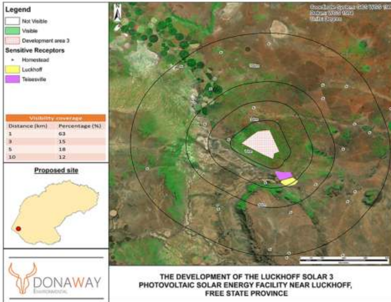
Figure 5.16: ZTV for the SEF, satellite view
