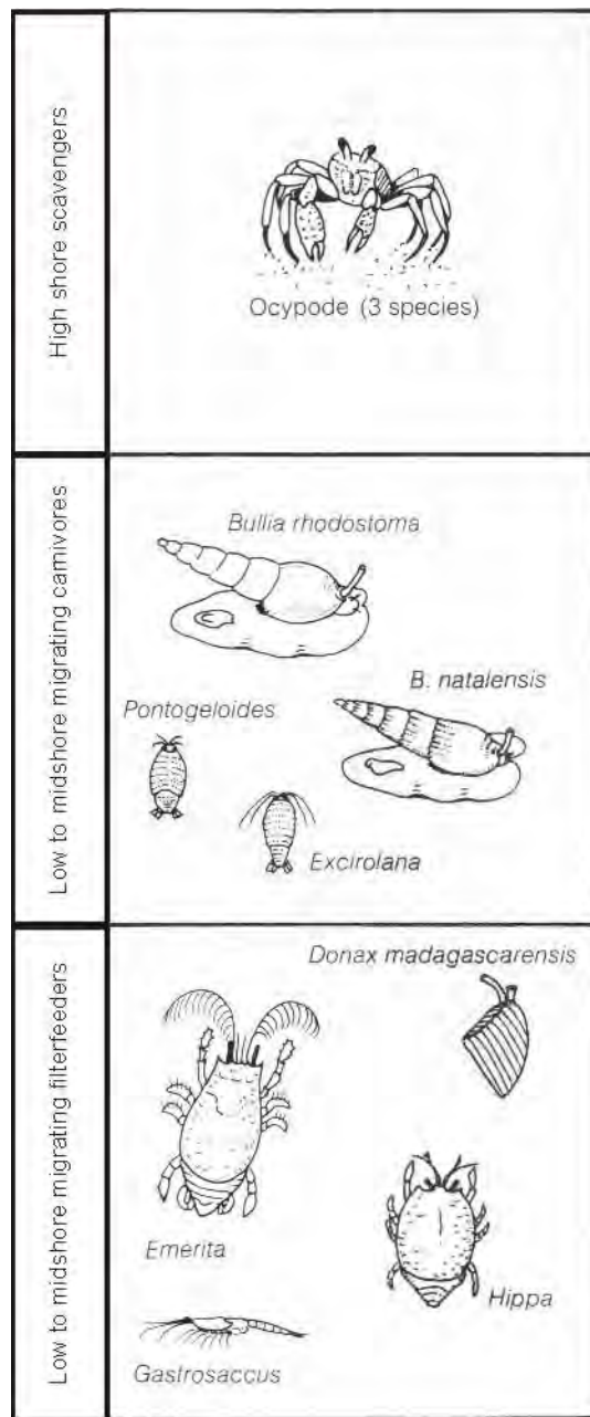
Figure 10: Schematic representation of the East Coast intertidal zonation on sandy beaches (adapted from Branch & Branch 1981).
