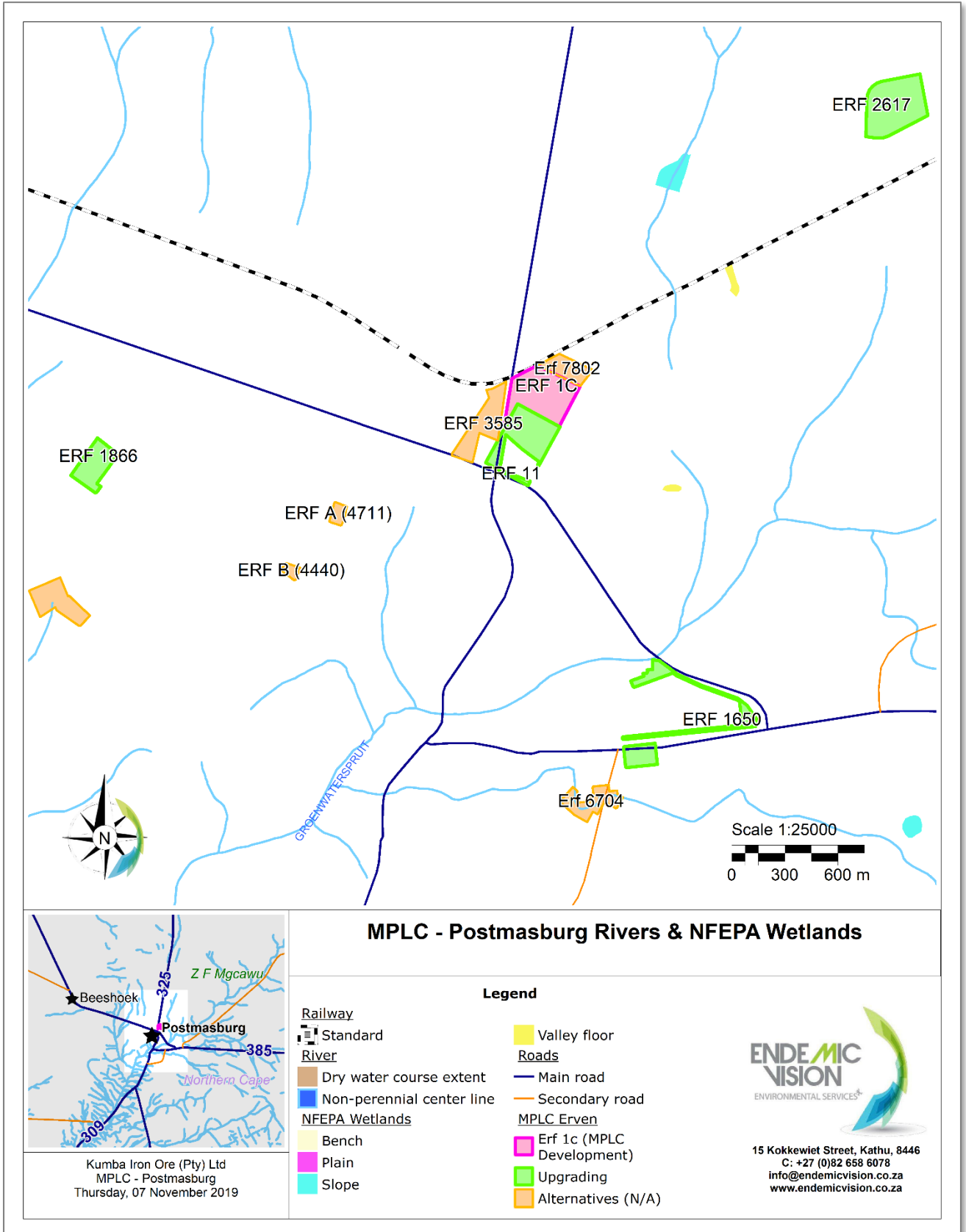
Figure 3: Rivers and NFEPA Wetlands
