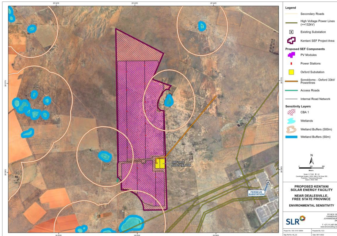
Figure 4-1: Project layout of the proposed Kentani Solar Energy Facility and environmental sensitivities
