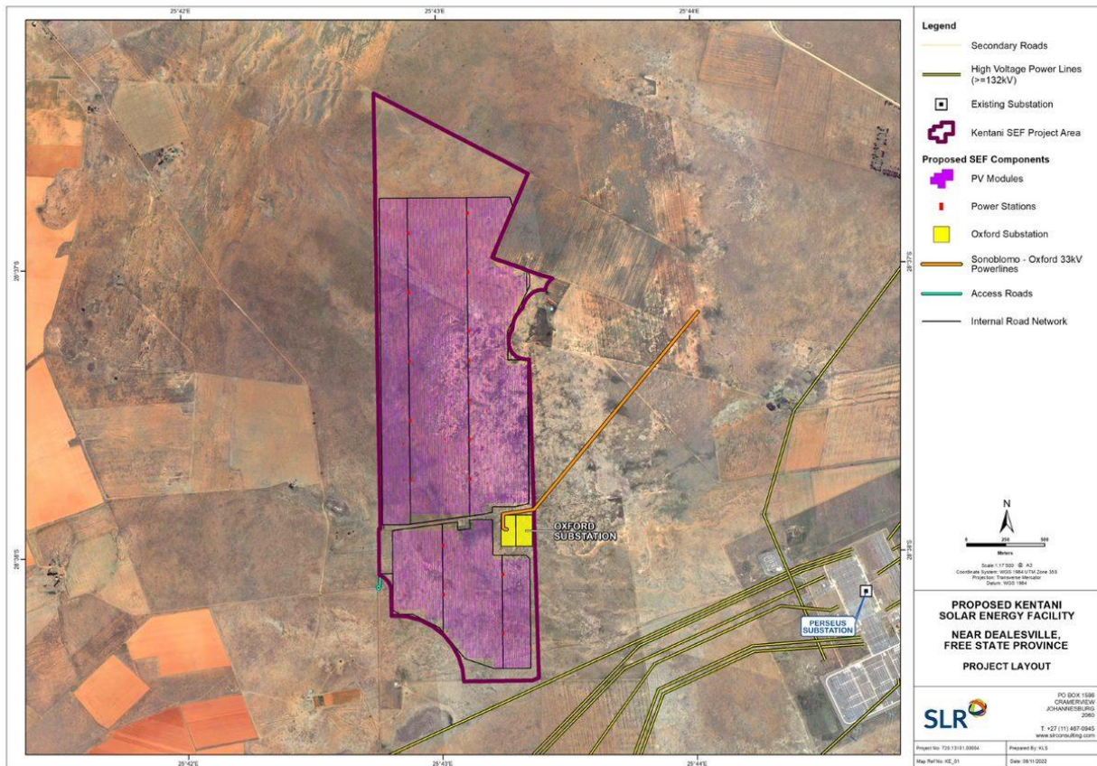
Figure 2: Project layout of the proposed Kentani Solar Facility
