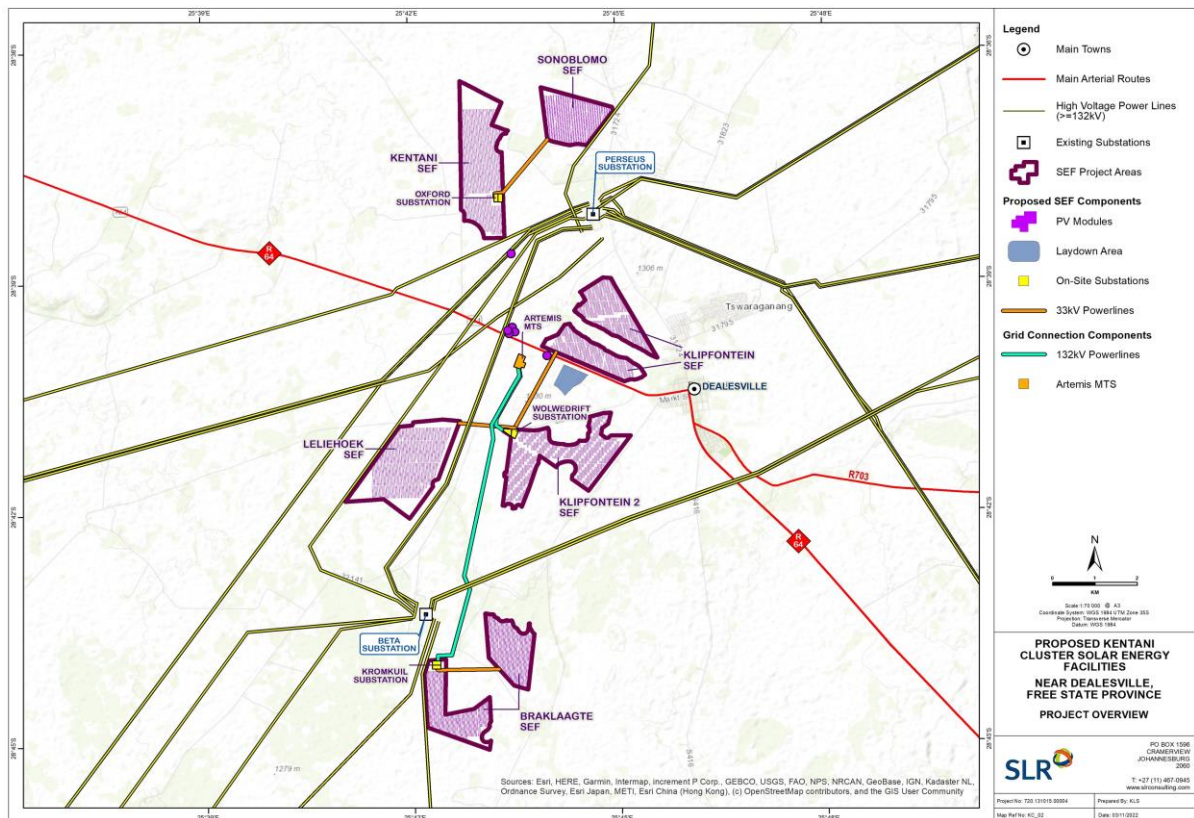
Figure 1-1: Locality map of the proposed Klipfontein SEF within the Kentani Cluster
