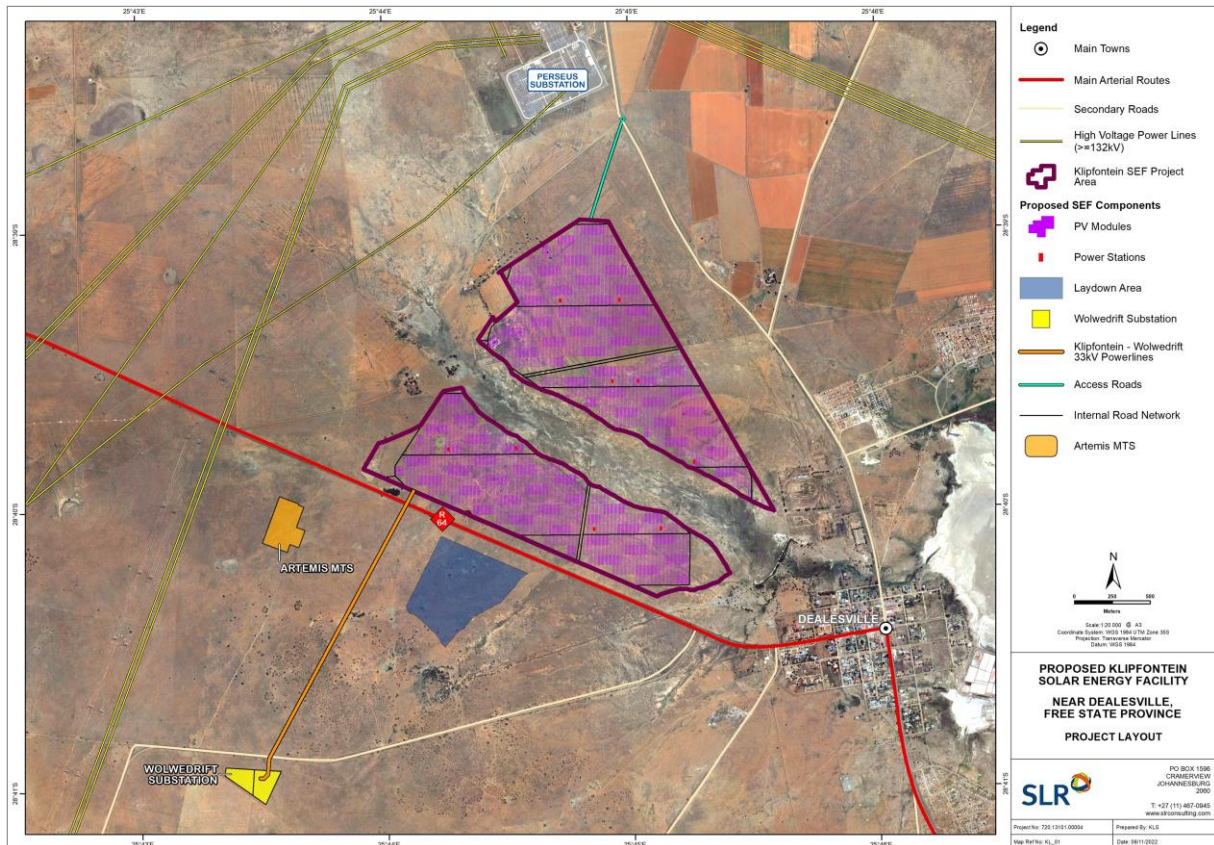
Figure 1-2: Layout map of the proposed Klipfontein SEF
