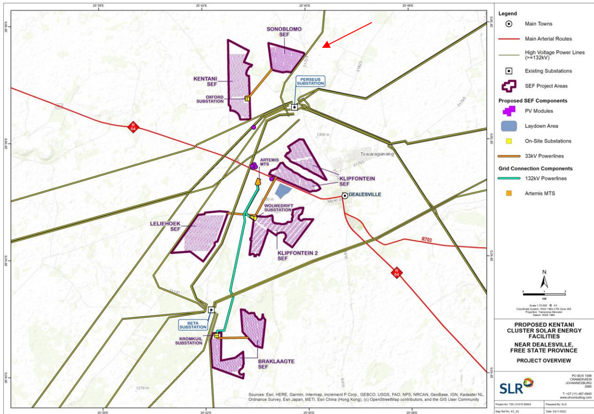
Figure 1-1: Project layout of the proposed Sonoblomo Solar Energy Facility
