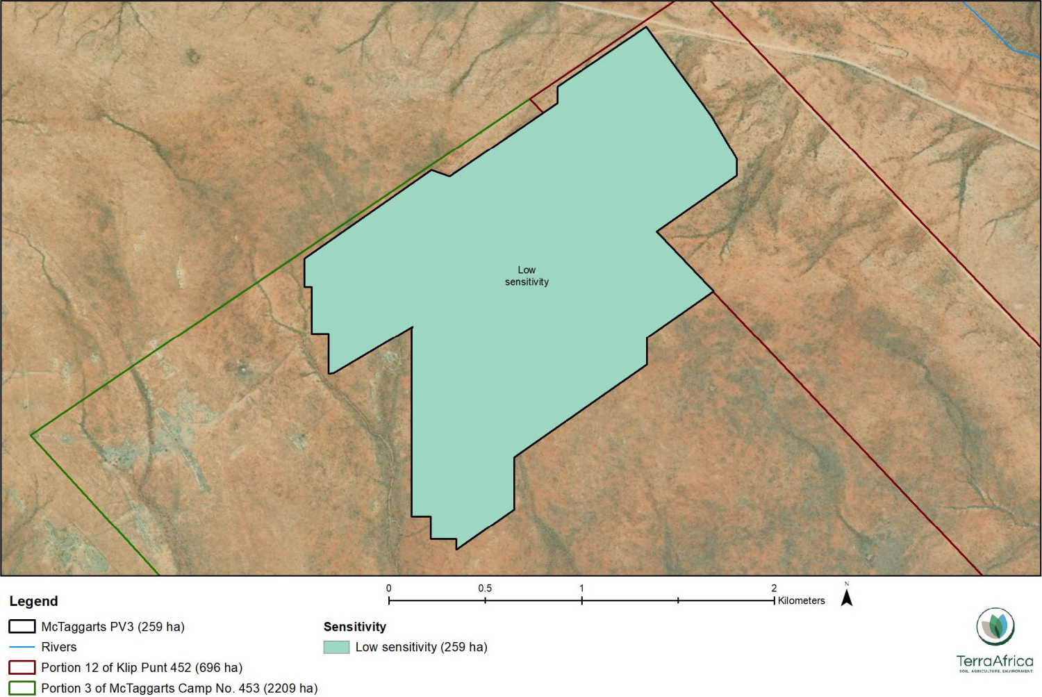
Figure 9: Sensitivity analysis of the baseline environment of the McTaggarts PV3 development area
