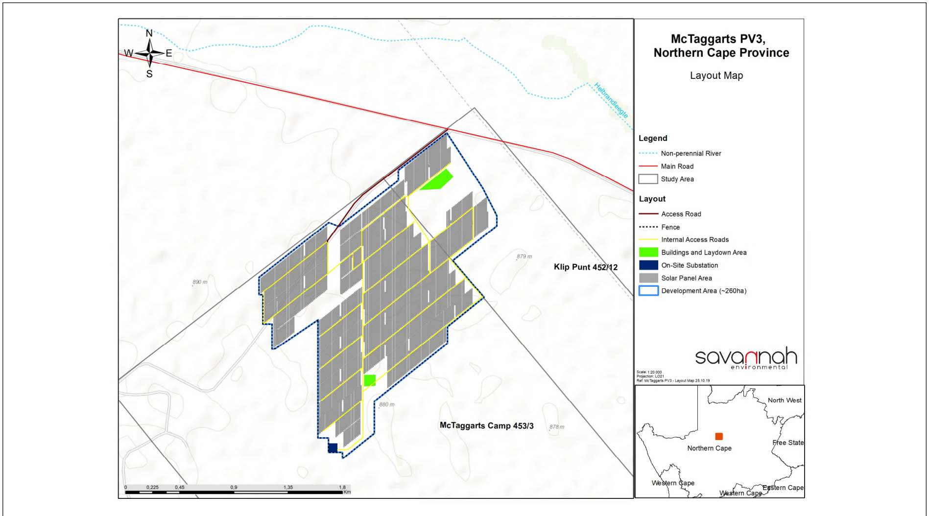
Figure 5.1: Facility layout of McTaggarts PV3 illustrating all infrastructure associated with the project
