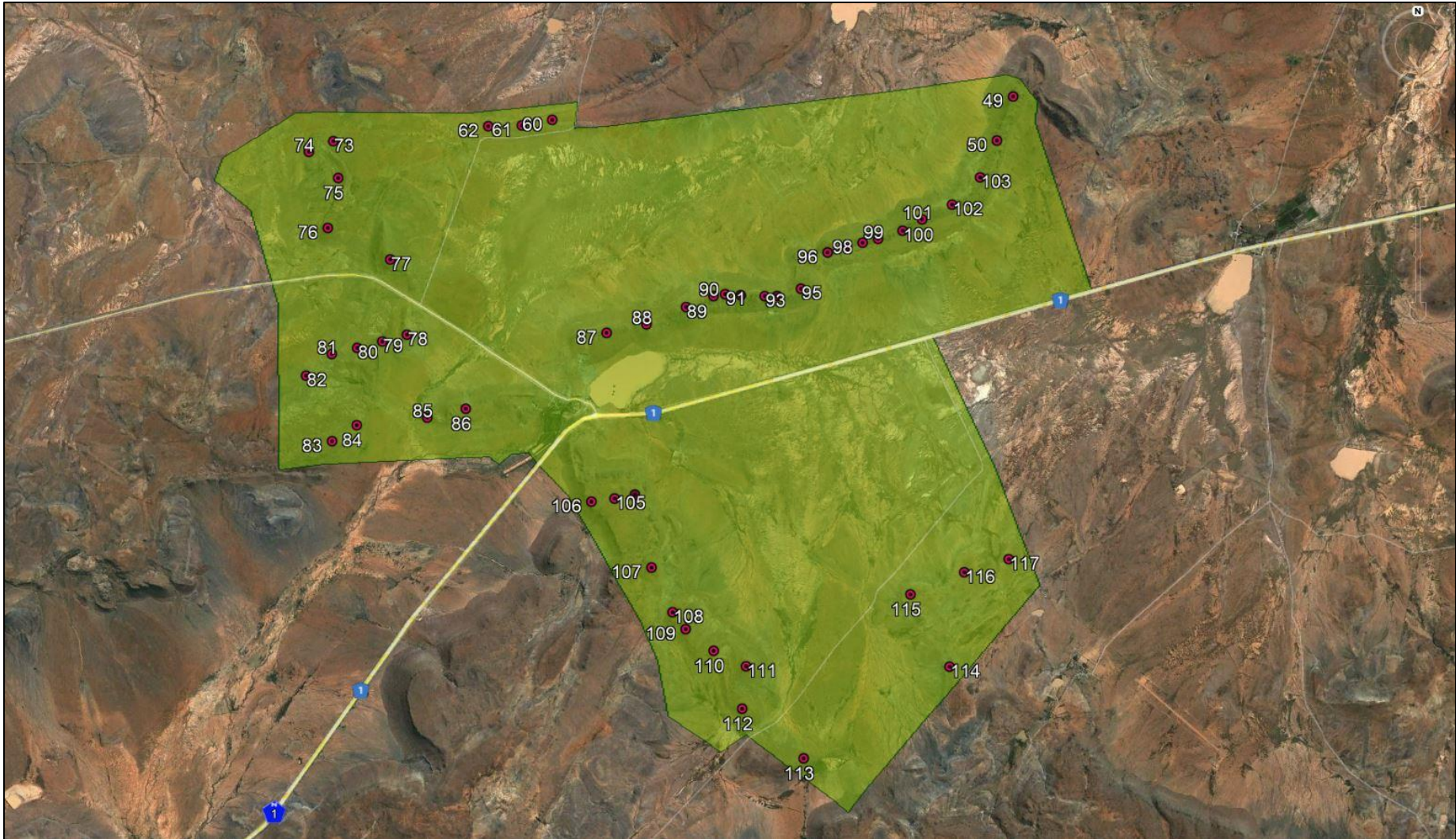
Figure 2.1. Preliminary turbine layout of the proposed Merino Wind Farm
