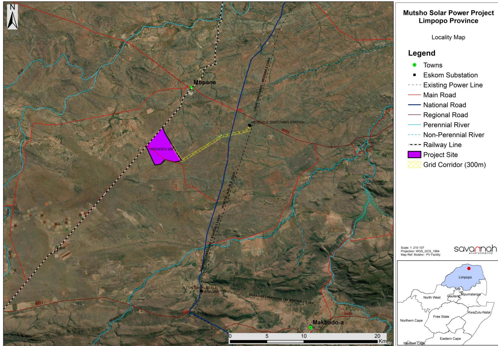
Figure 2.1: Locality map of the project site within which Mutsho Solar PV3 is proposed to be developed.
