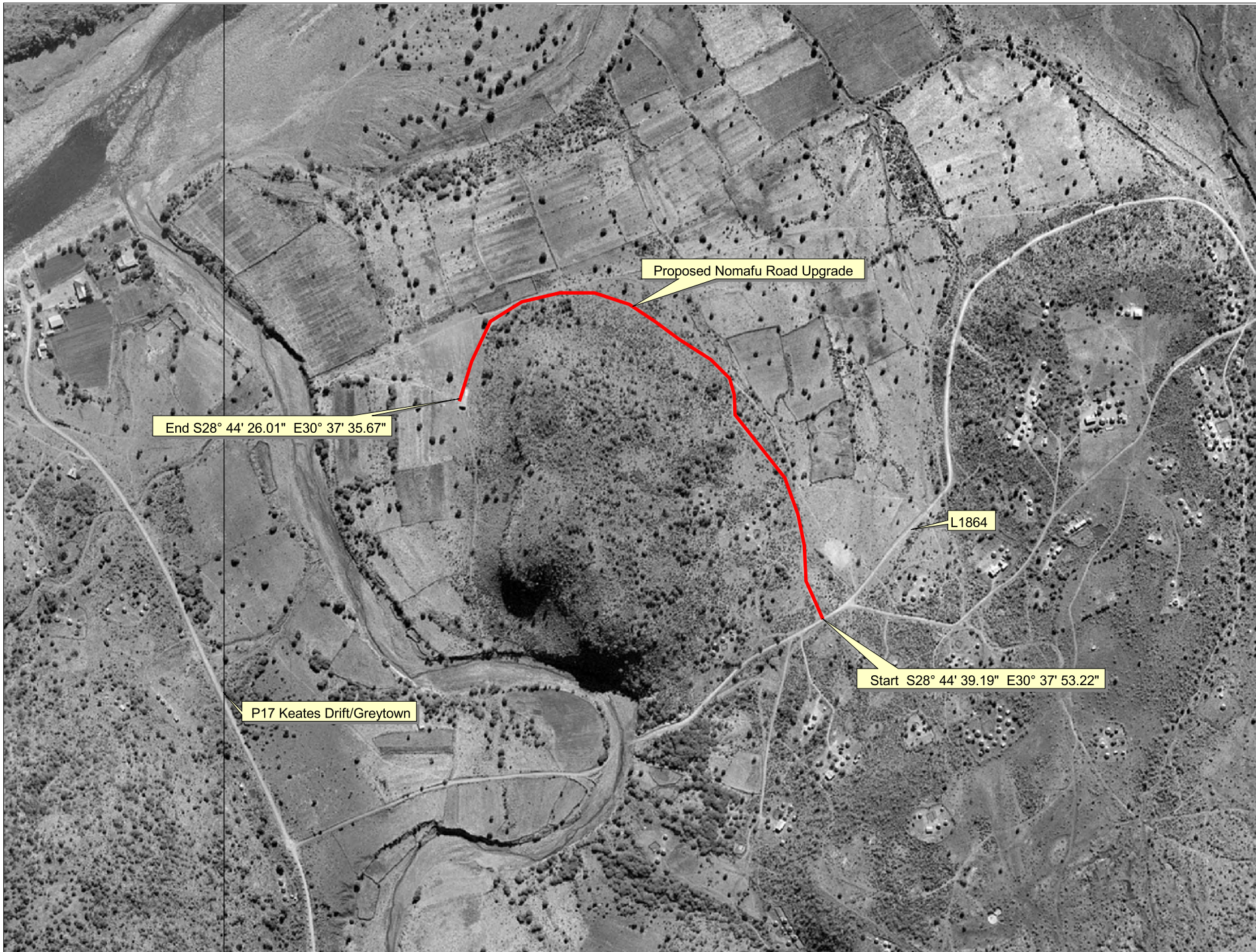
Proposed Nomafu Road Upgrade
