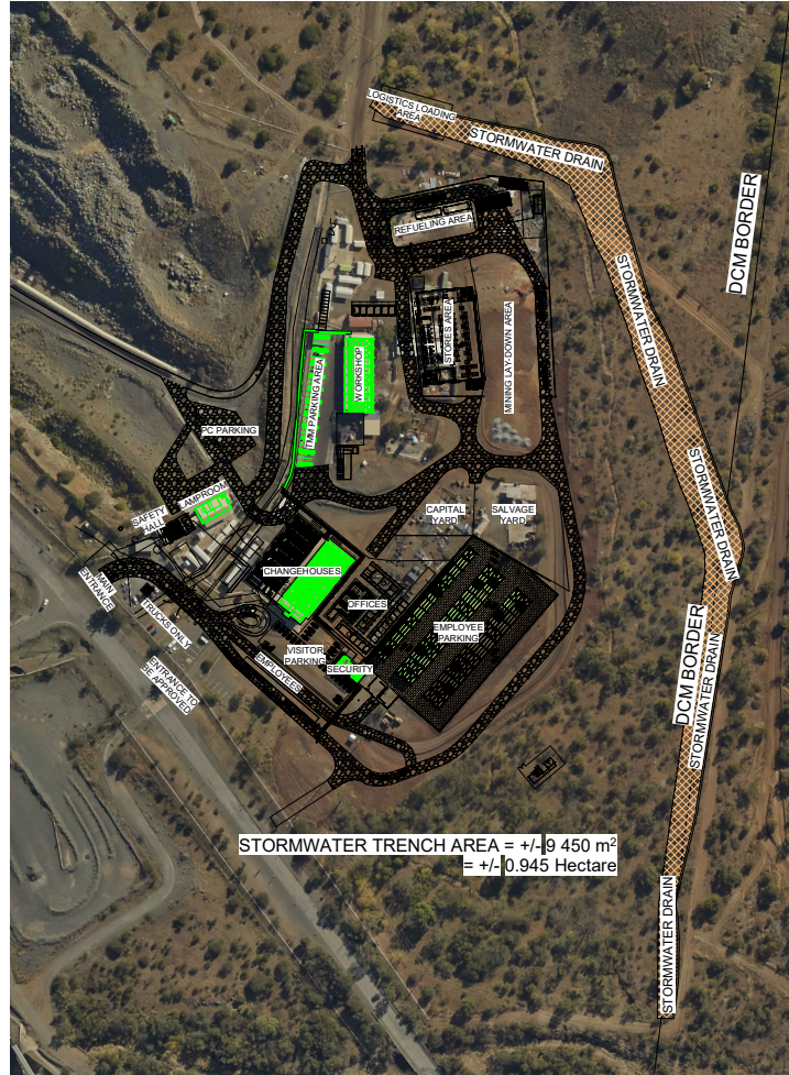
1 Site Plan Showing Stormwater trench 1:1000
