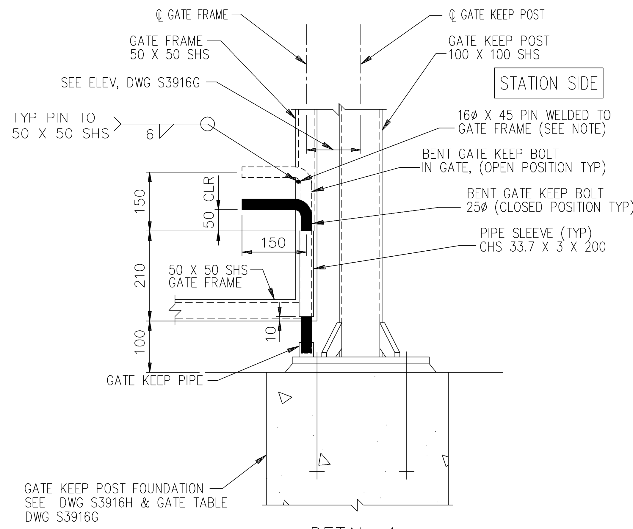
DETAIL 4 INSIDE ELEVATION OF SINGLE SWING GATE KEEP NTS
