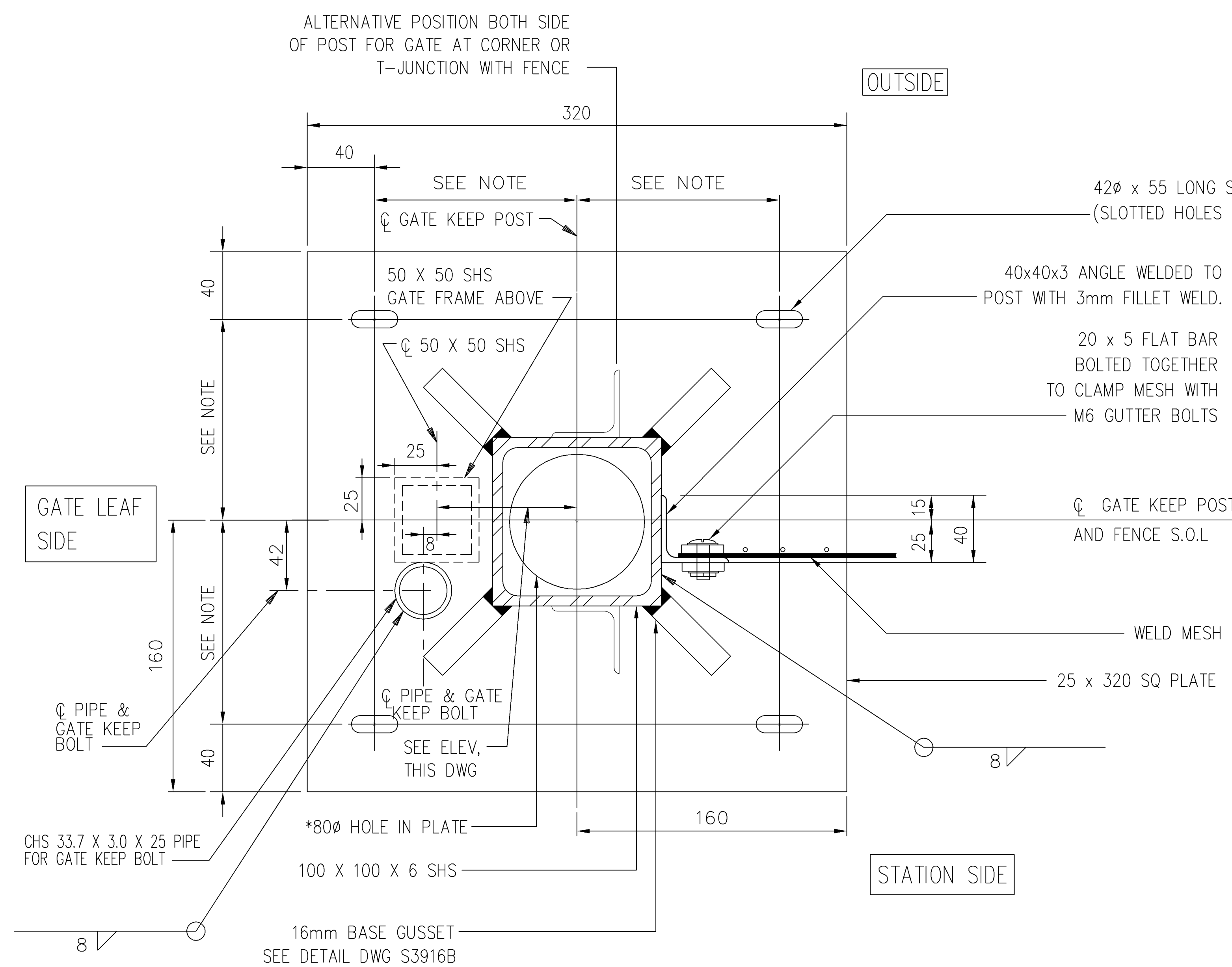
DETAIL 5 PLAN OF GATE KEEP POST BASE PLATE (TYP)(SEE NOTE) (FOR SINGLE SWING GATES 11 & 12 ONLY) NTS
