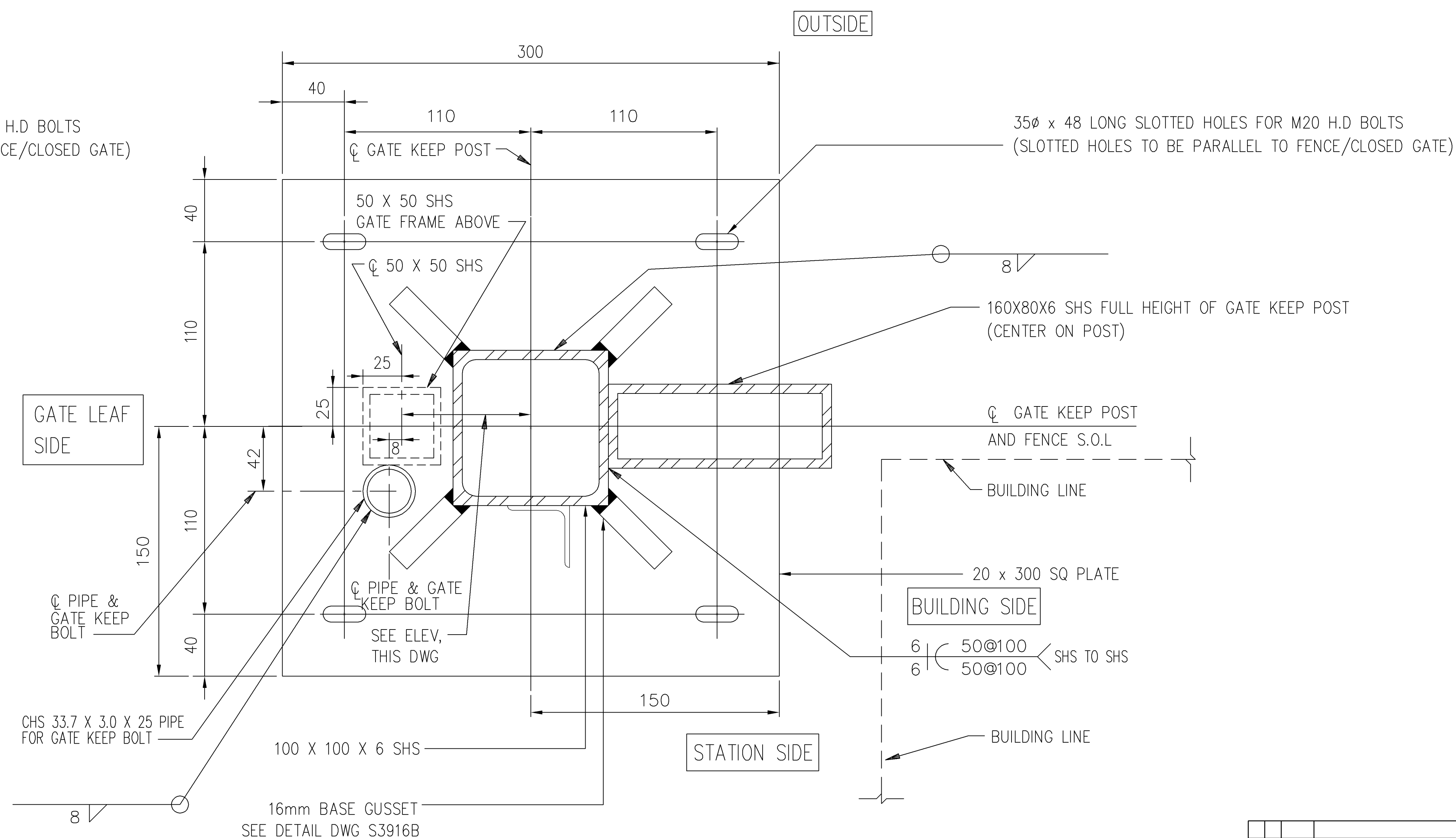
DETAIL 5A PLAN OF GATE KEEP POST BASE PLATE ADJACENT TO BUILDING (FOR SINGLE SWING GATE 14)(SEE NOTES) NTS
