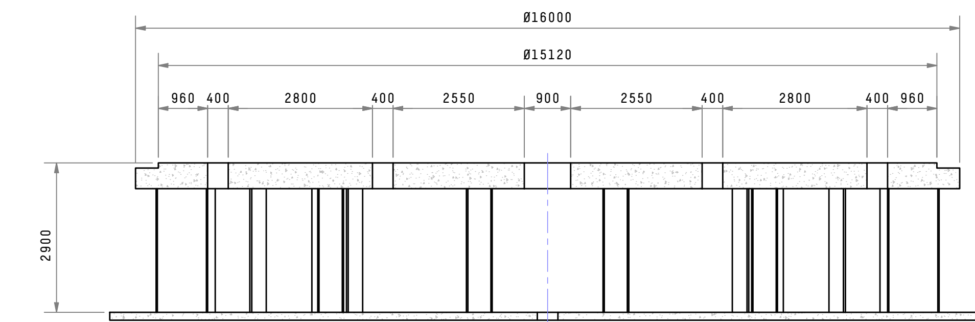
Section R-R
