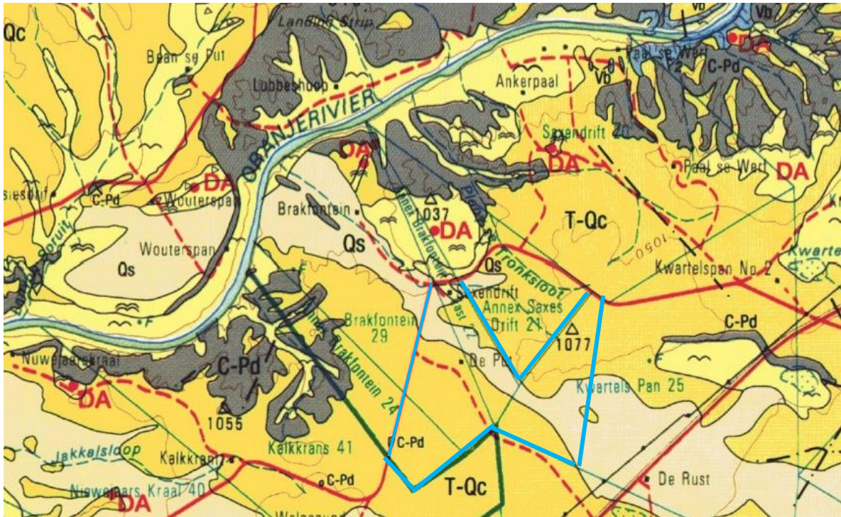
Figure 4: Geological map of the area around the Farm Brakfontein 276 RE with the location of the proposed project indicated within the turquoise polygon. Abbreviations of the rock types are explained in Table 2. Map enlarged from the Geological Survey 1: 250 000 map 2922 Prieska.
