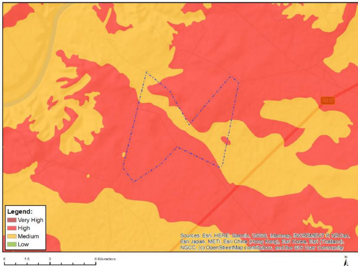
Figure 6: DFFE Screening palaeosensitivity map – high for the Tertiary calcretes and medium for the Quaternary sands and Dwyka Group.
