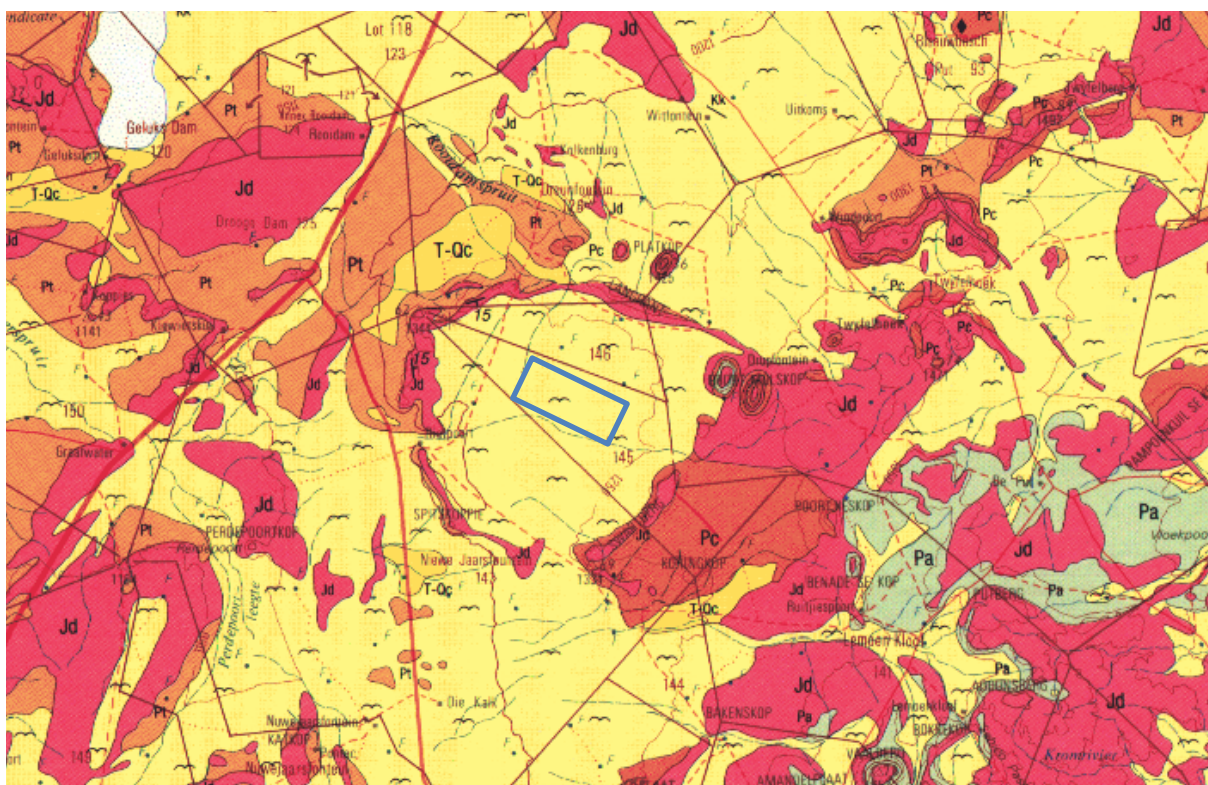
Figure 3: Geological map of the area around the Soyuz 1 Solar PV Park. The location of the proposed project is indicated within the blue rectangle. Abbreviations of the rock types are explained in Table 2. Map enlarged from the Geological Survey 1: 250 000 map 3022 Britstown.
