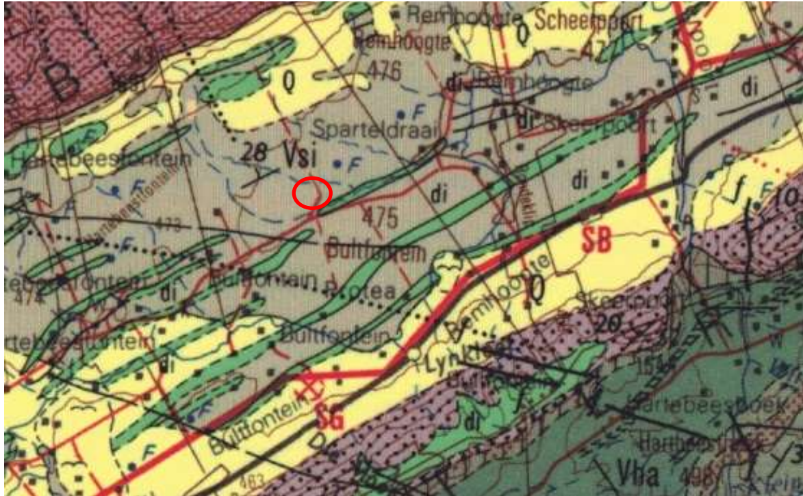
Figure 3: Geological map of the area around the Farm Bultfontein 475 JQ with the proposed site for the Vodacom mast shown within the red outline on rocks of the Silverton Formation (symbol Vsi, grey). Abbreviations of the rock types are explained in Table 2. Map enlarged from the Geological Survey 1: 250 000 map 2526 Rustenburg.
