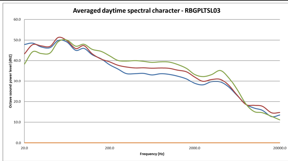
Figure 6-25: Average daytime frequencies - RBGPLTSL03
