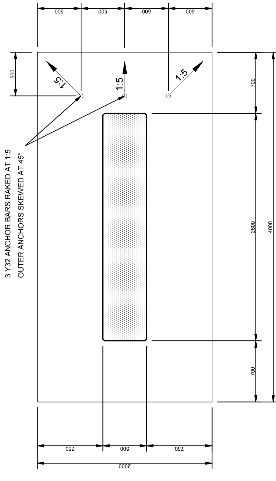
PLAN OF CENTRE PIER BASE 1:25
