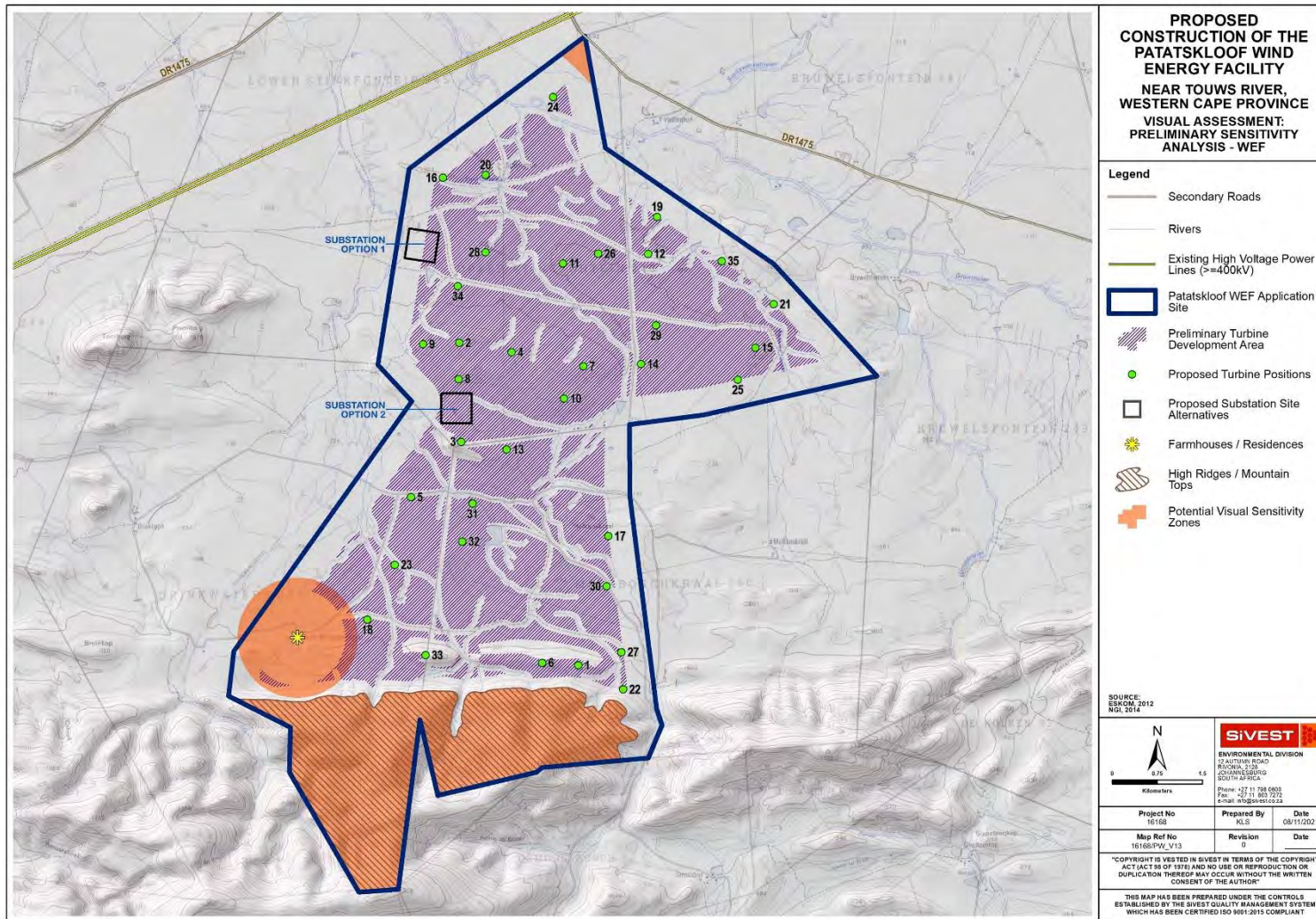
Figure 25: Visual sensitivity on the Patatskloof WEF Site
