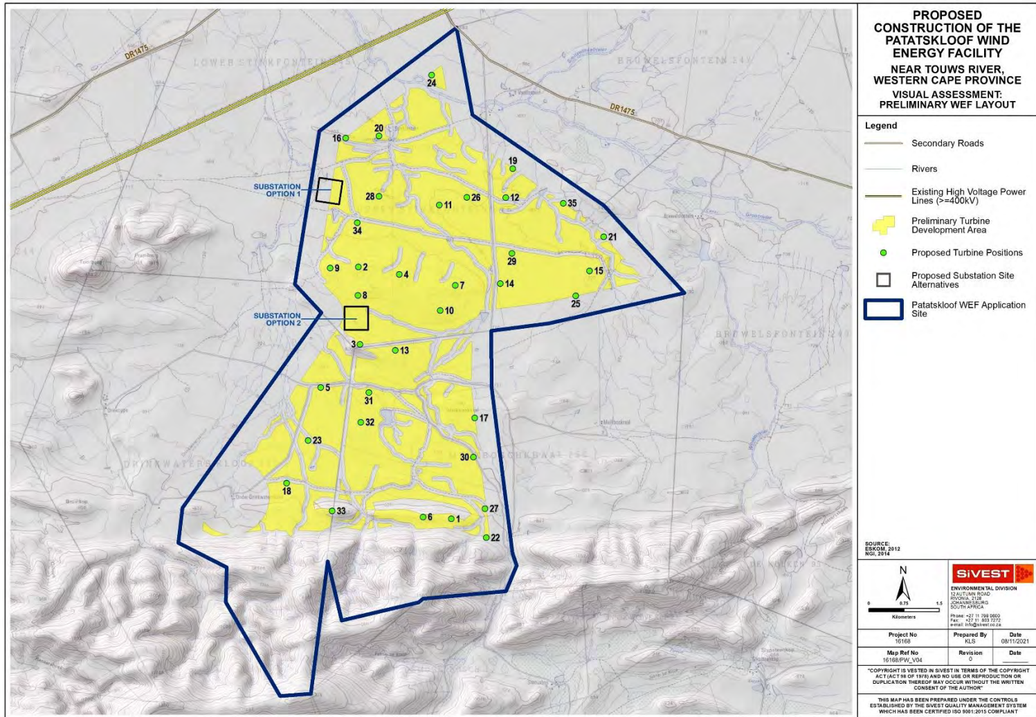
Figure 5: Preliminary Patatskloof WEF layout
