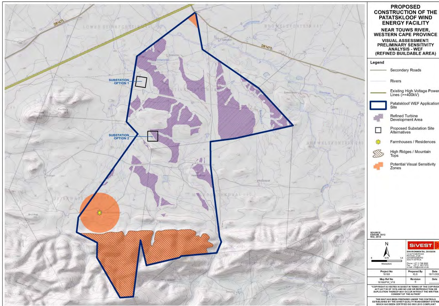
Figure 34: Refined Buildable Area
