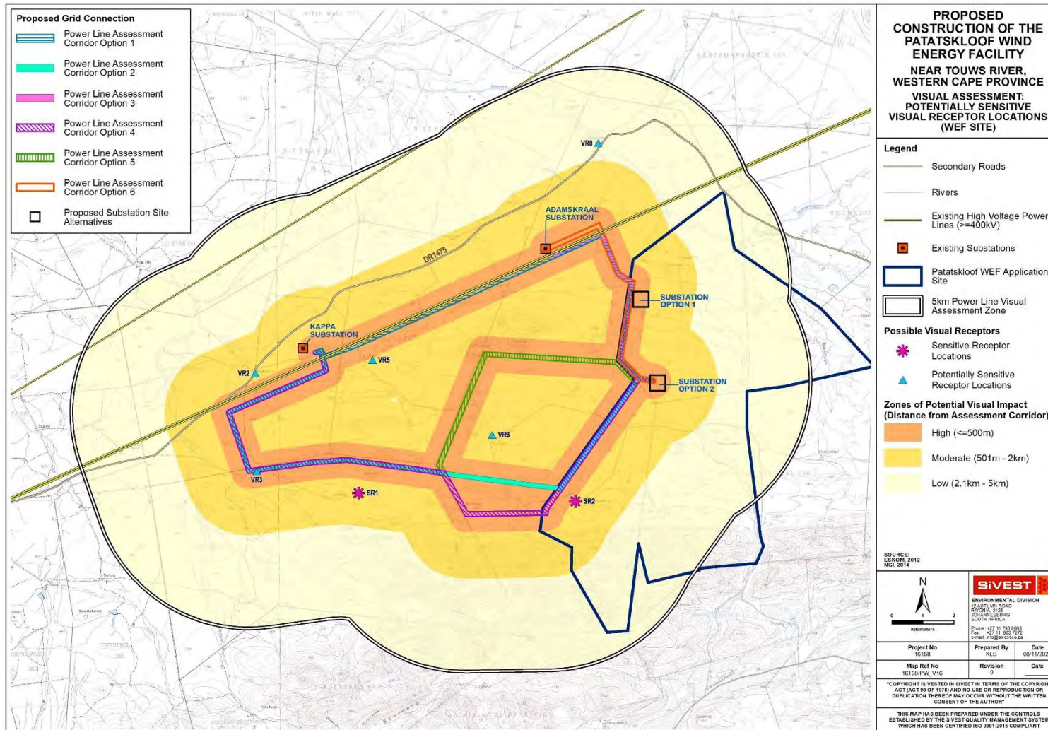
Figure 31: Potentially sensitive receptor locations within 5kms of the power line corridor
