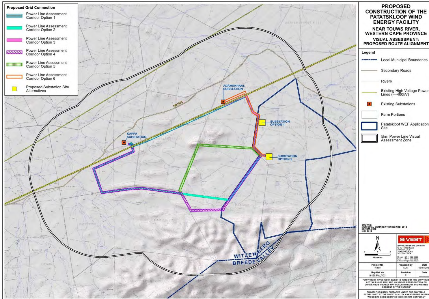
Figure 3: Proposed 132kV Power Line Route Overview
