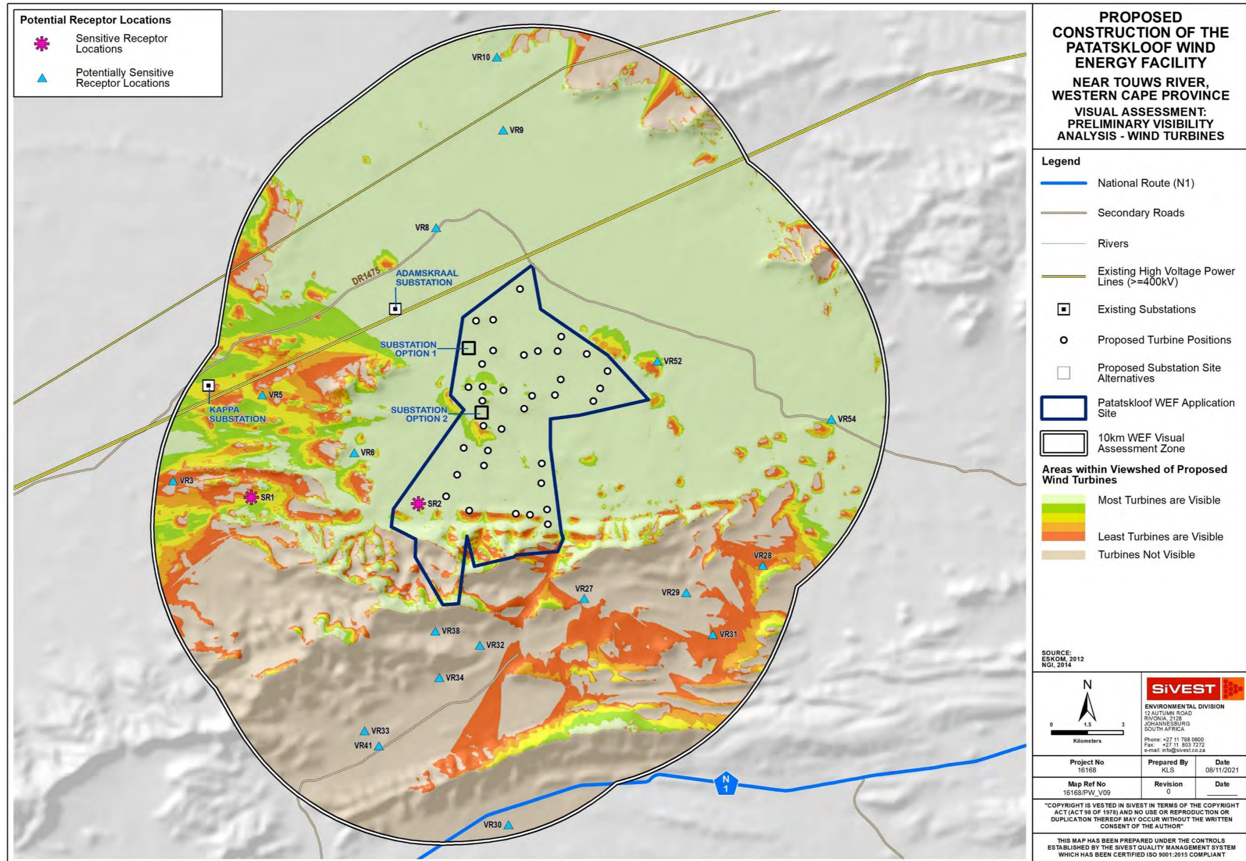
MAP 9: Potential Visibility of Wind Turbines
