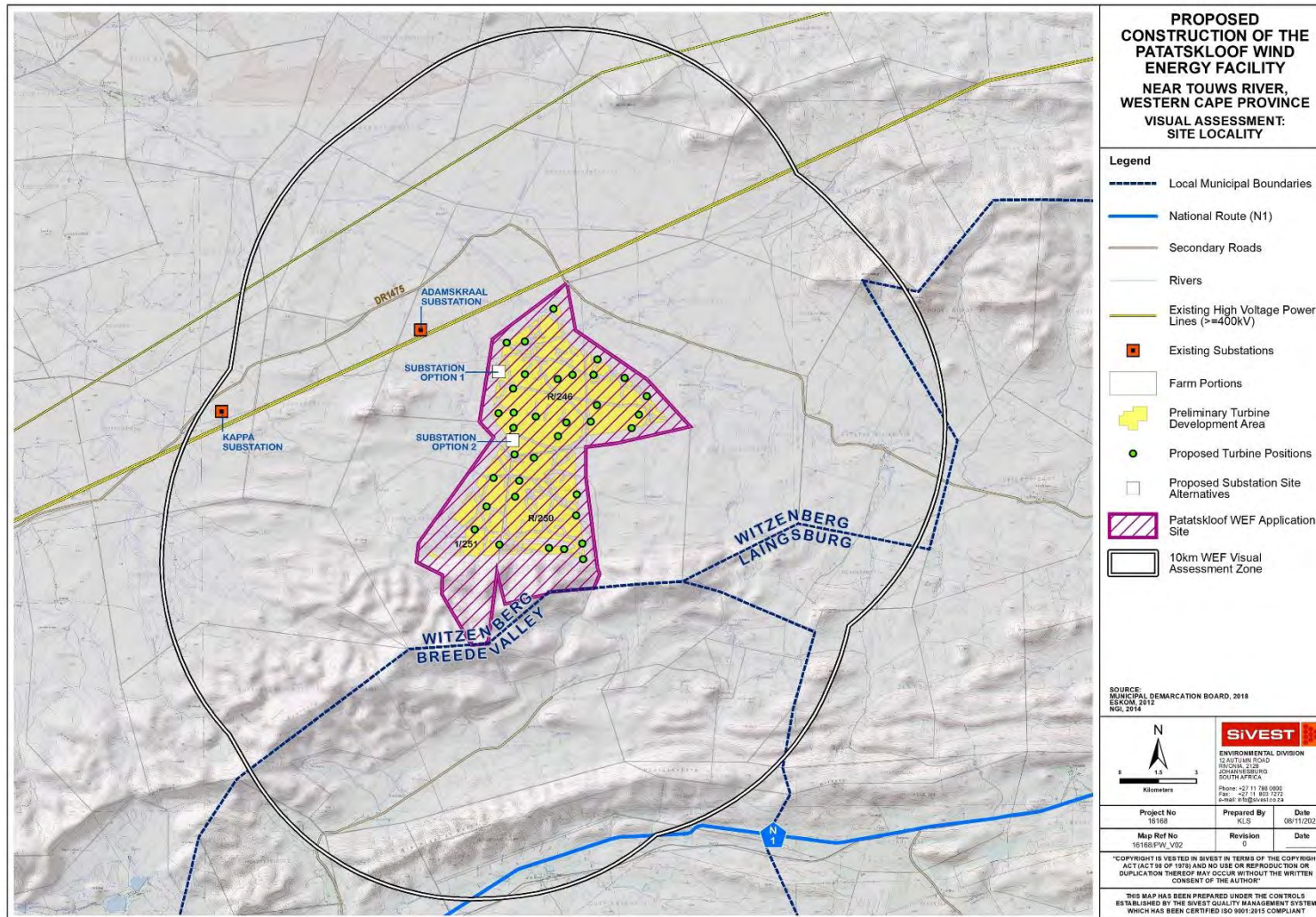
Figure 2: Patatskloof WEF Site Locality
