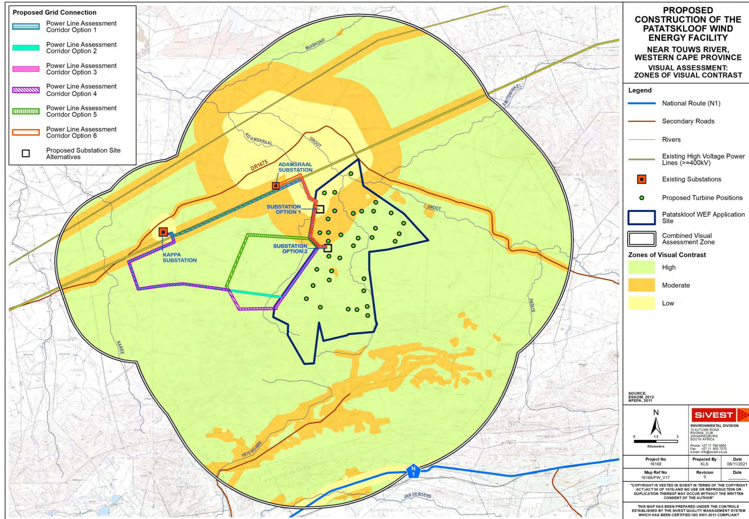
MAP 17: Zones of Visual Contrast in the Combined Study Area
