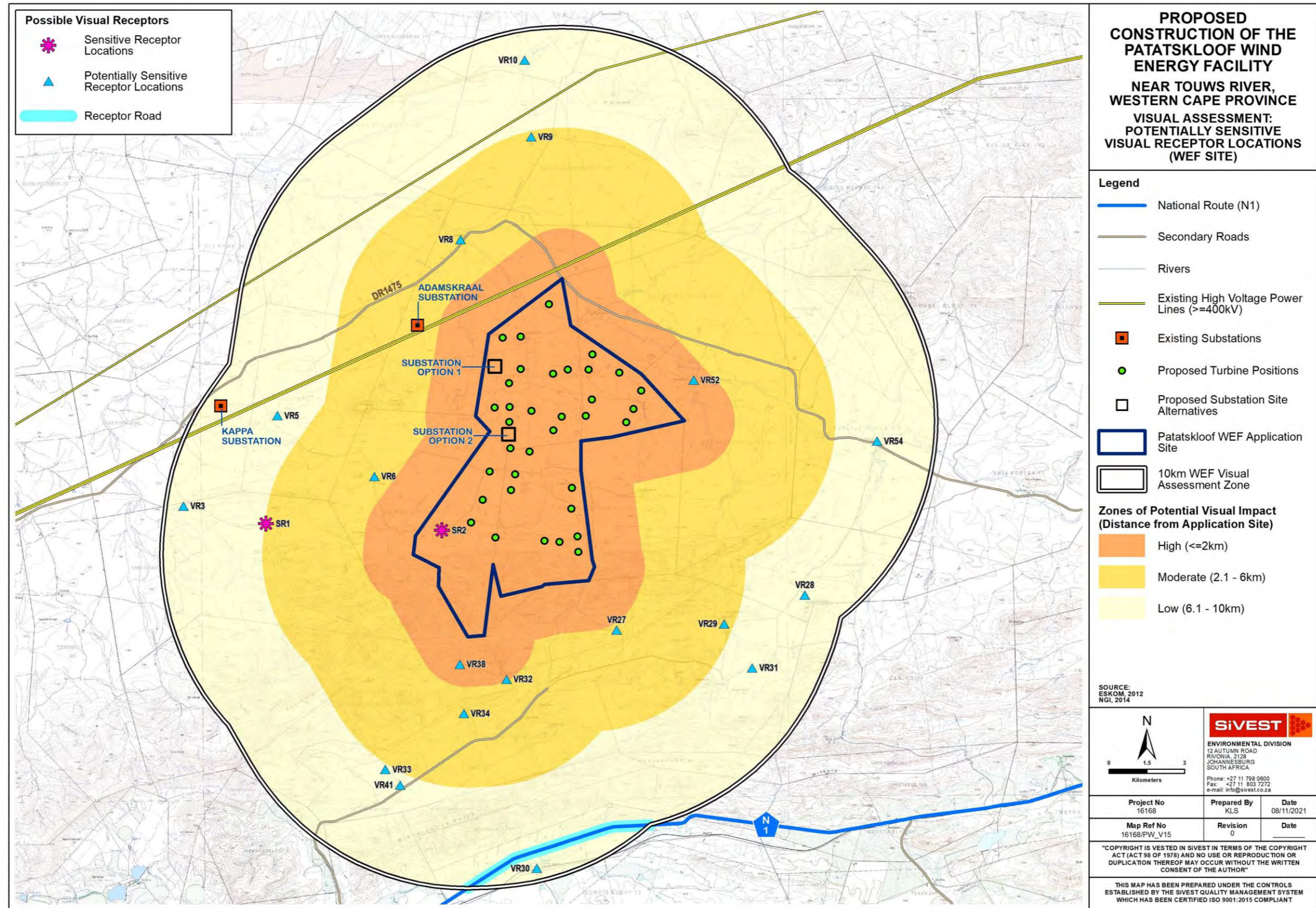
MAP 15: Potentially Sensitive Receptor Locations within 10kms of the Patatskloof WEF Application Site
