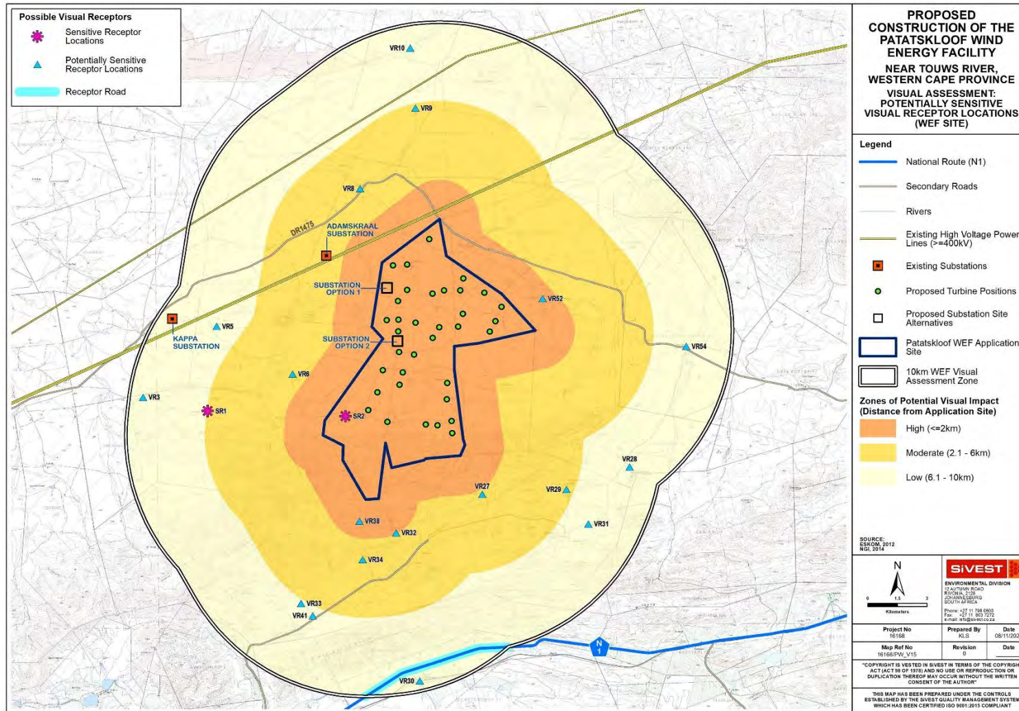
Figure 30: Potentially sensitive receptor locations within 10kms of the Patatskloof WEF application site
