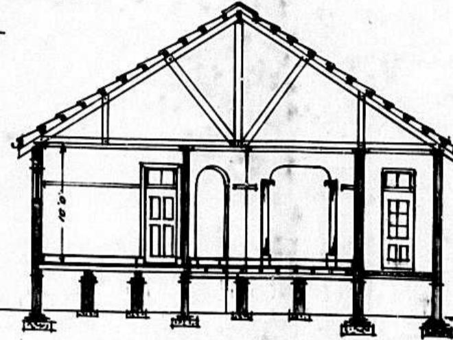
CROSS SECTION
