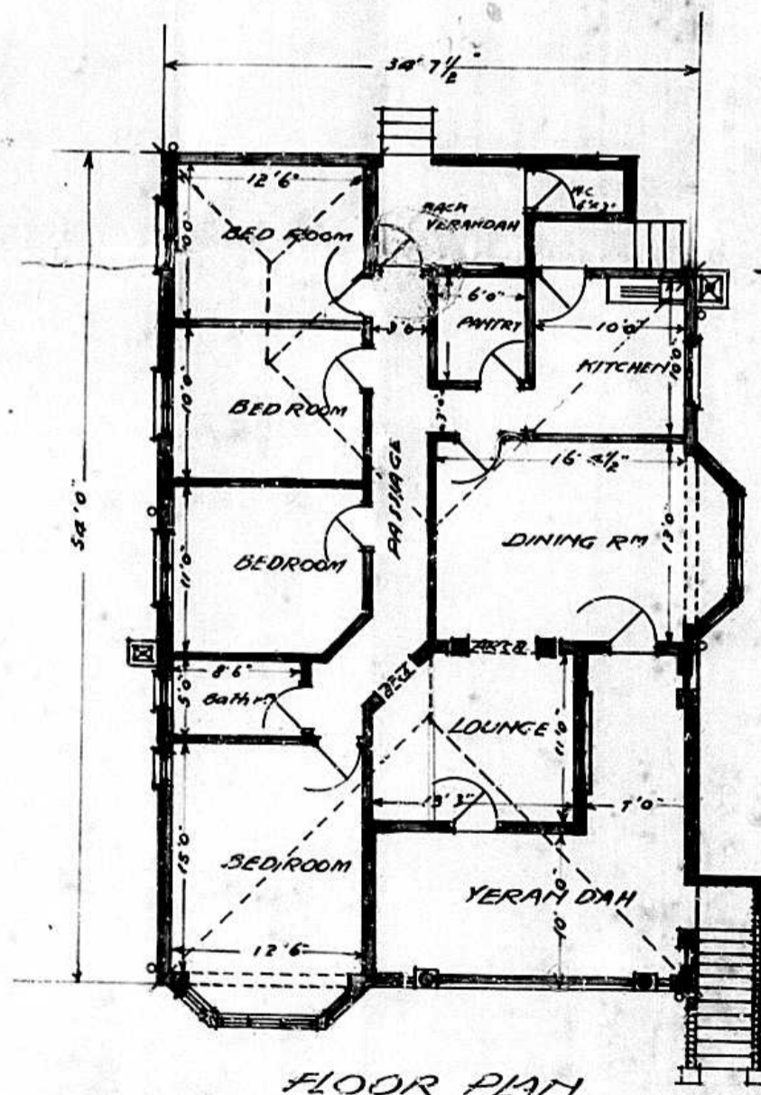
FLOOR PLAN
