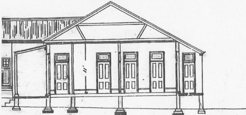
Section Scale 1/4" = 1' for 1"
