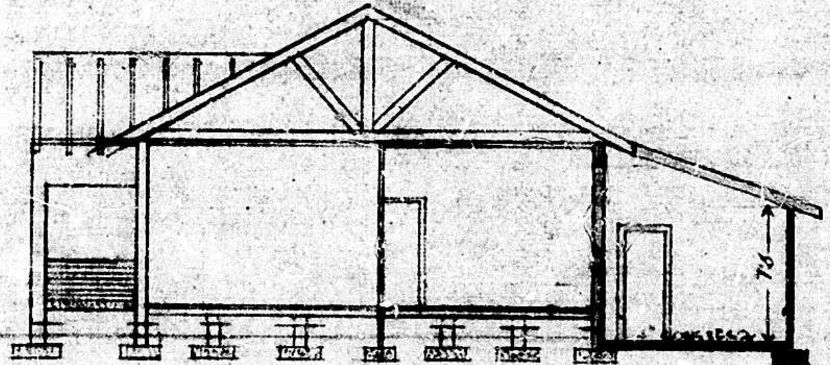
CROSS SECTION
