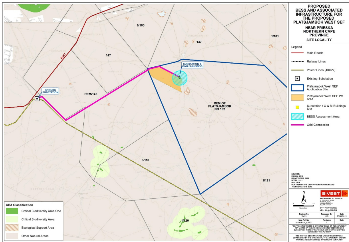
Figure 1: BESS is located on the authorised Platsjambok West Photovoltaic (PV) Energy Facility
