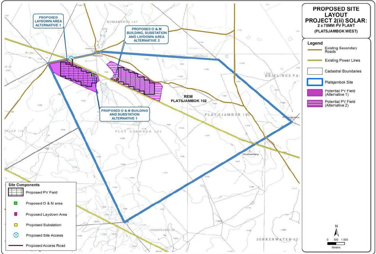
Figure 3 Previous watercourse study developable area and preferred site location
