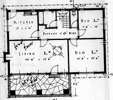
GROUND PLAN
