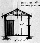
PLAN & SECTION C-D OF OUTBUILDING.
