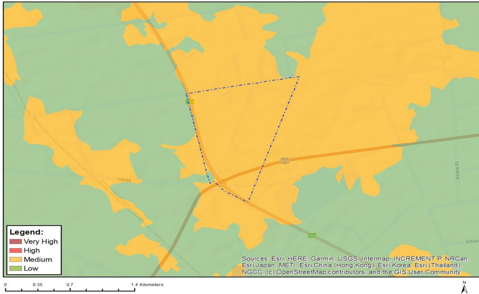
Figure 10: Map of relative plant species theme sensitivity
