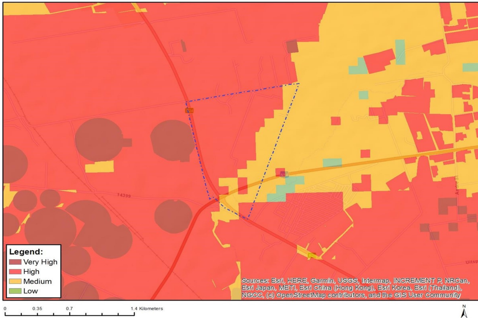
Figure 2: Map of relative agriculture theme sensitivity
