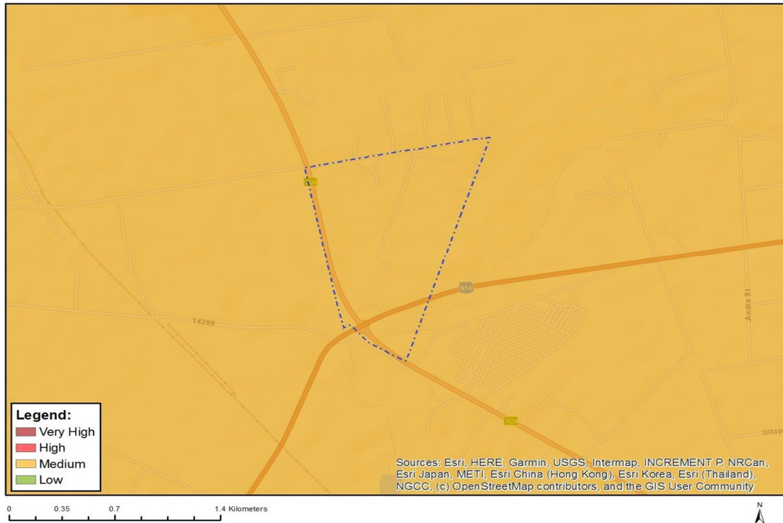
Figure 7: Map of relative civil aviation theme sensitivity
