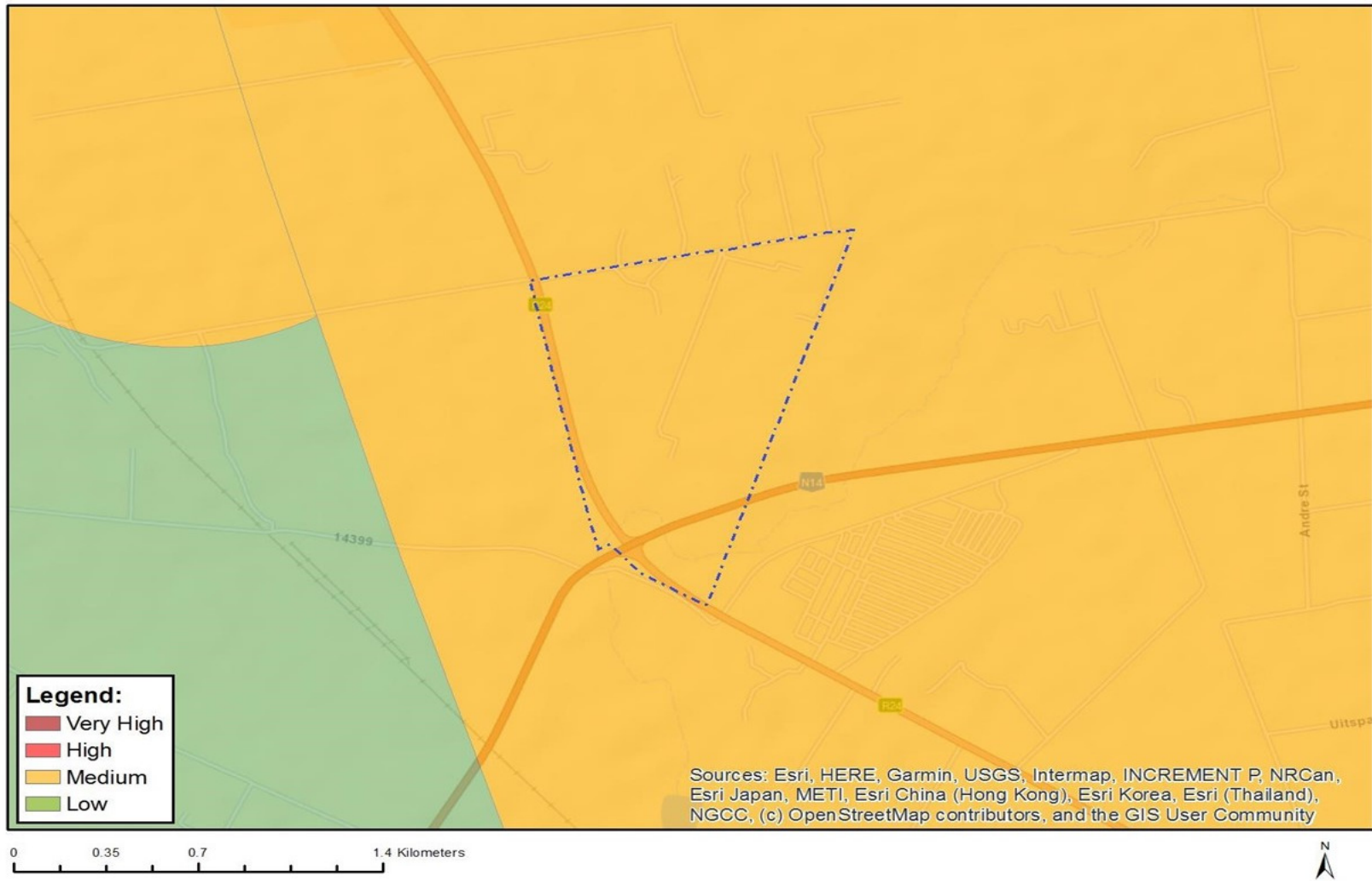
Figure 11: Map of relative RFI theme sensitivity
