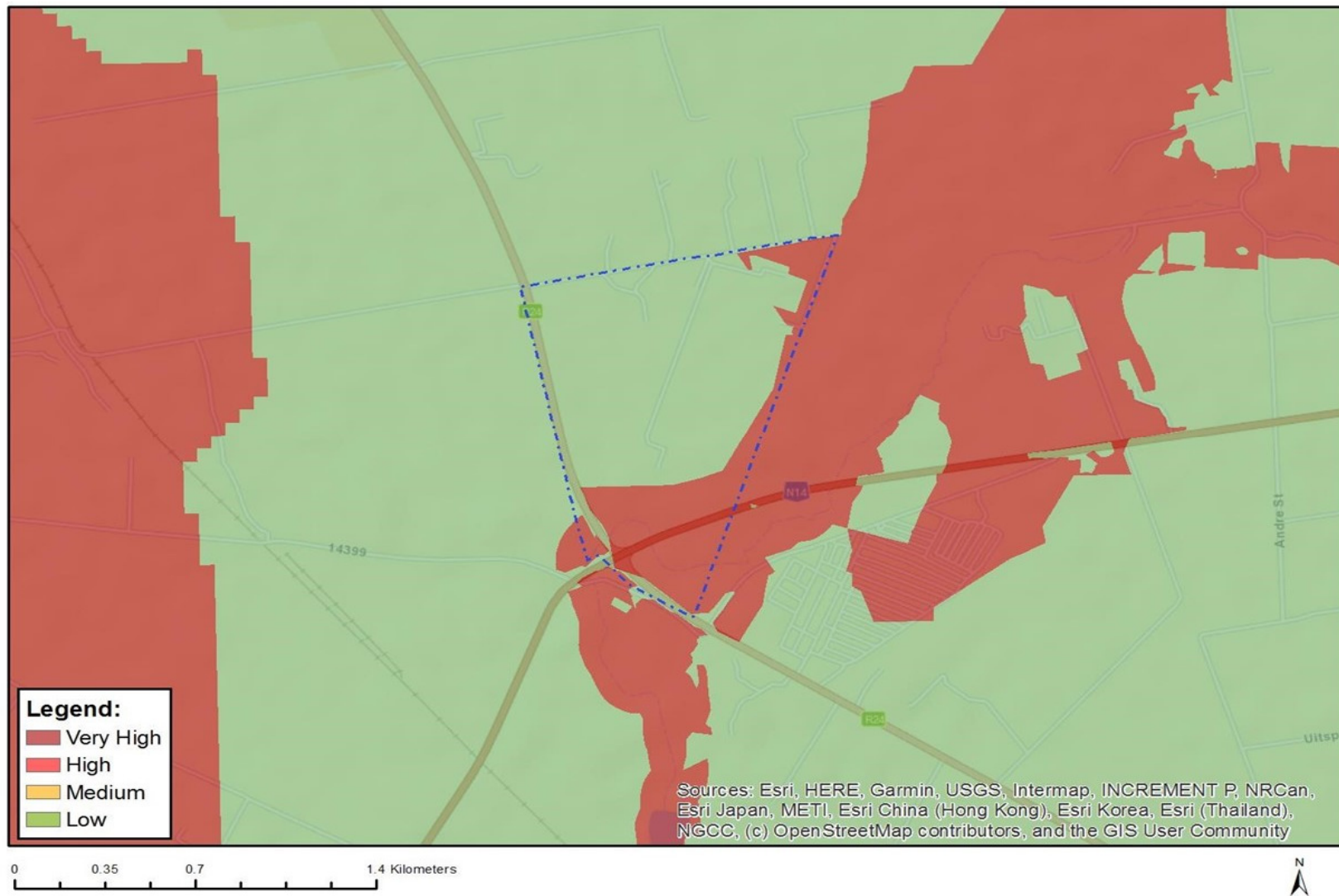
Figure 12: Map of relative terrestrial biodiversity theme sensitivity
