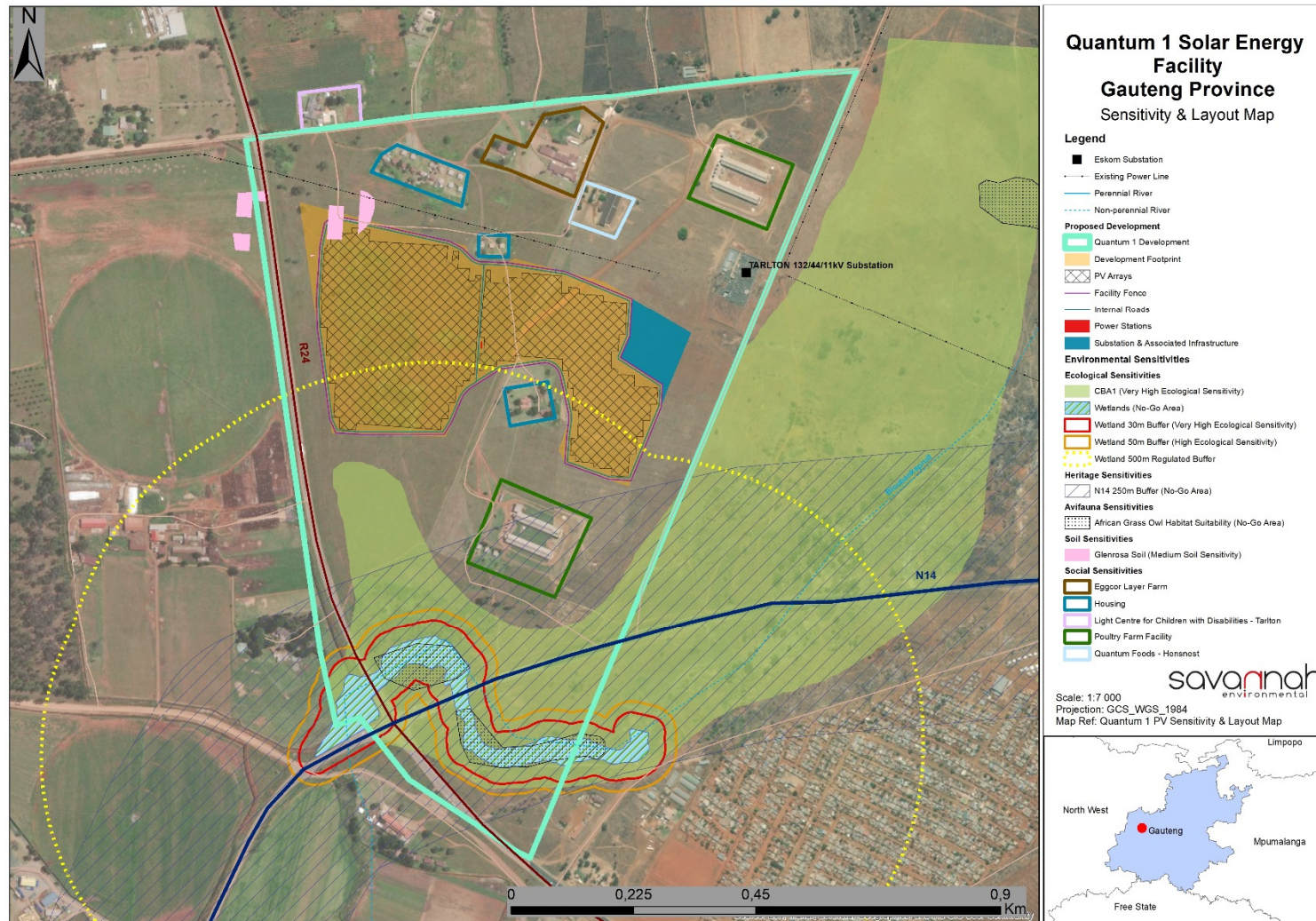
Figure 1: Sensitivity map of the development footprint of the Quantum PV Facility
